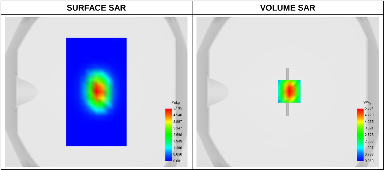
Maximum location: X=2.00, Y=1.00 ; SAR Peak: 8.76 W/kg
