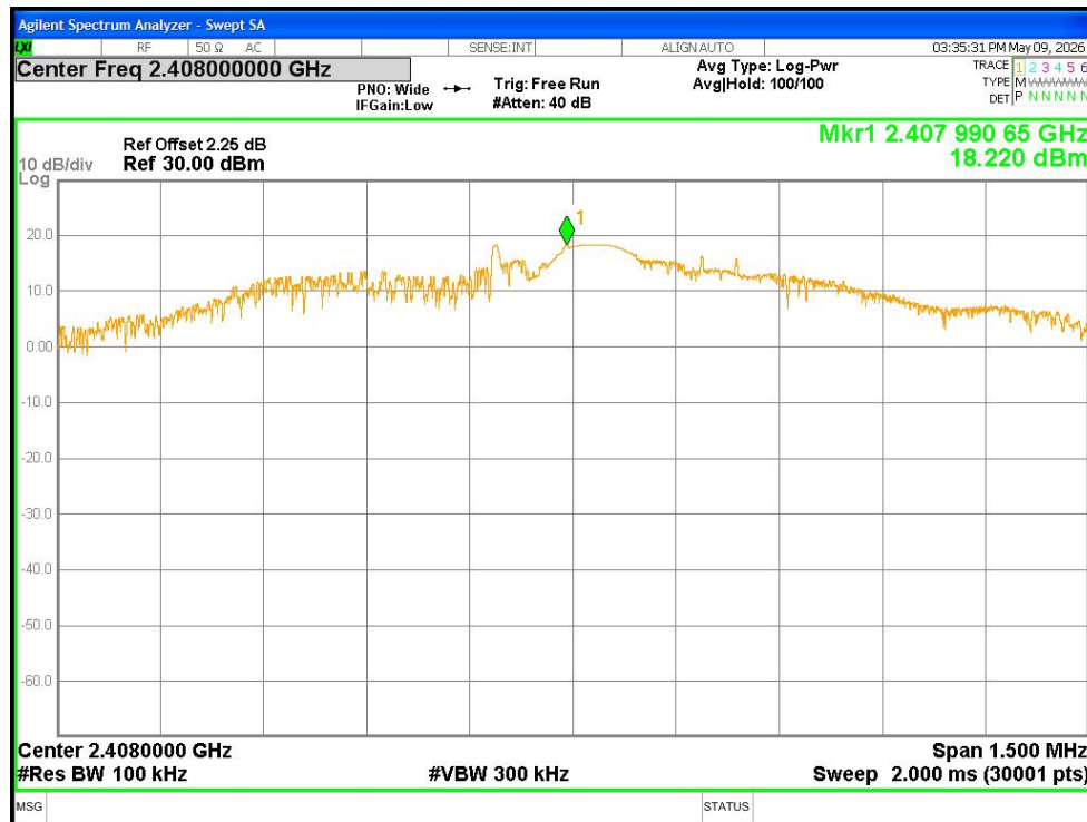
Tx. Spurious NVNT 2.4G 2408MHz Ant1 Emission
