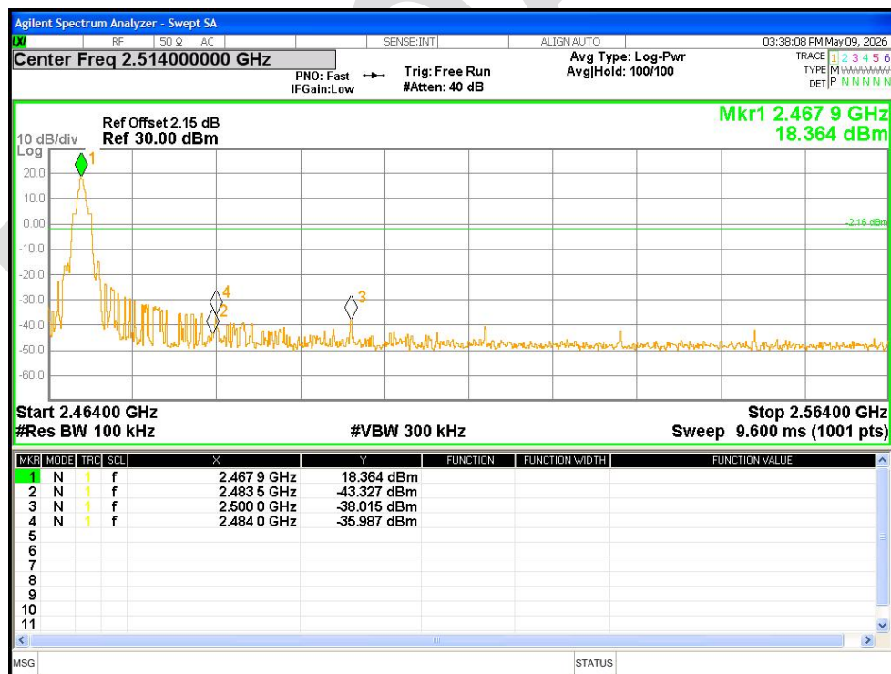
Band Edge NVNT 2.4G 2468MHz Ant1 No-Hopping Emission
