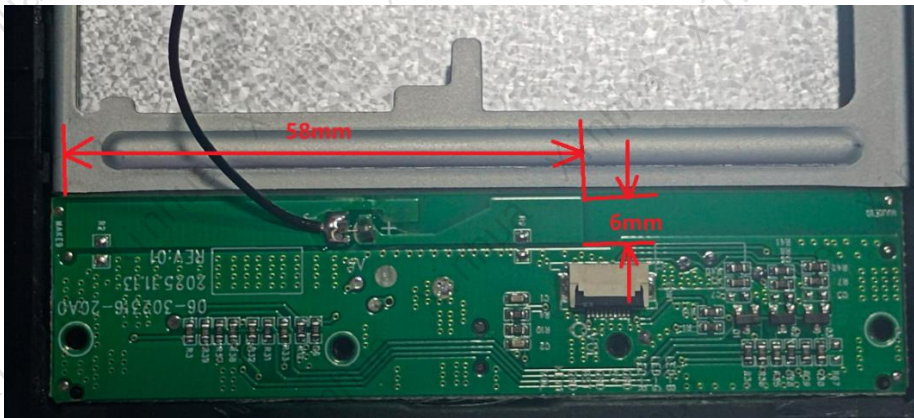
Antenna Dimensions
