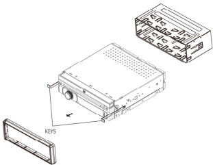
TYPICAL FRONT-LOAD DIN MOUNTING METHOD
