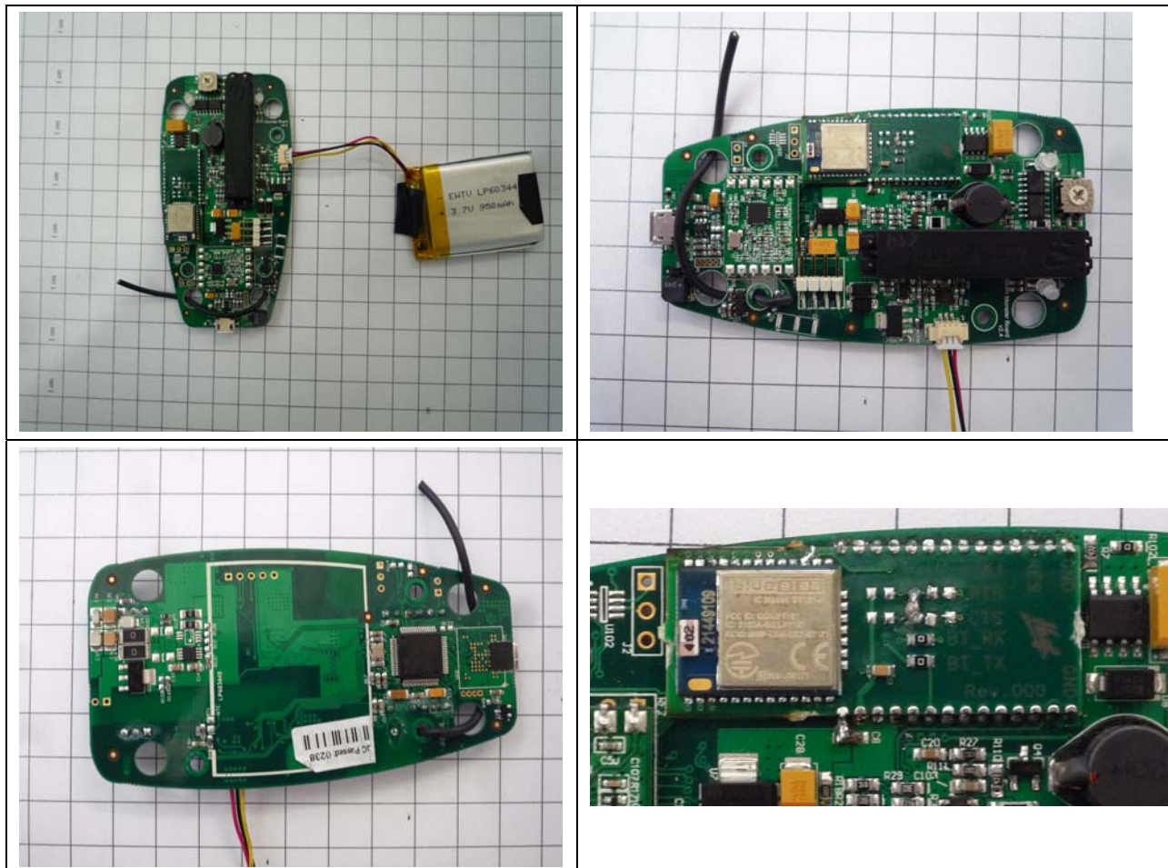
Photograph 3: EUT identification – internal view
