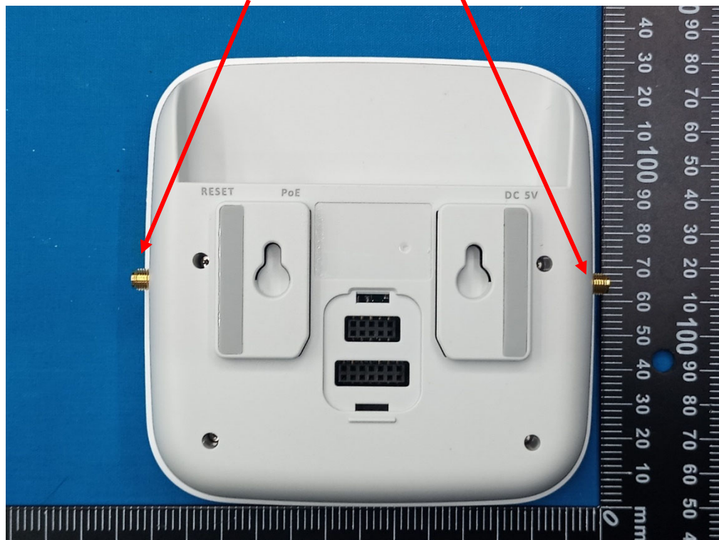
Antenna 1 (RT) / Antenna 2 (AP)
