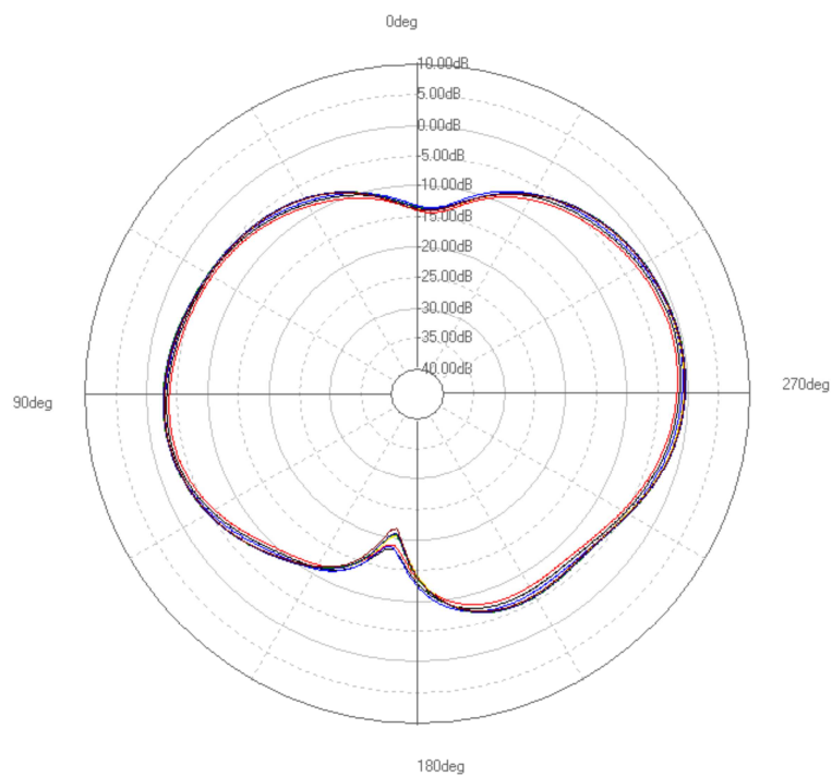
X-Z Plane
