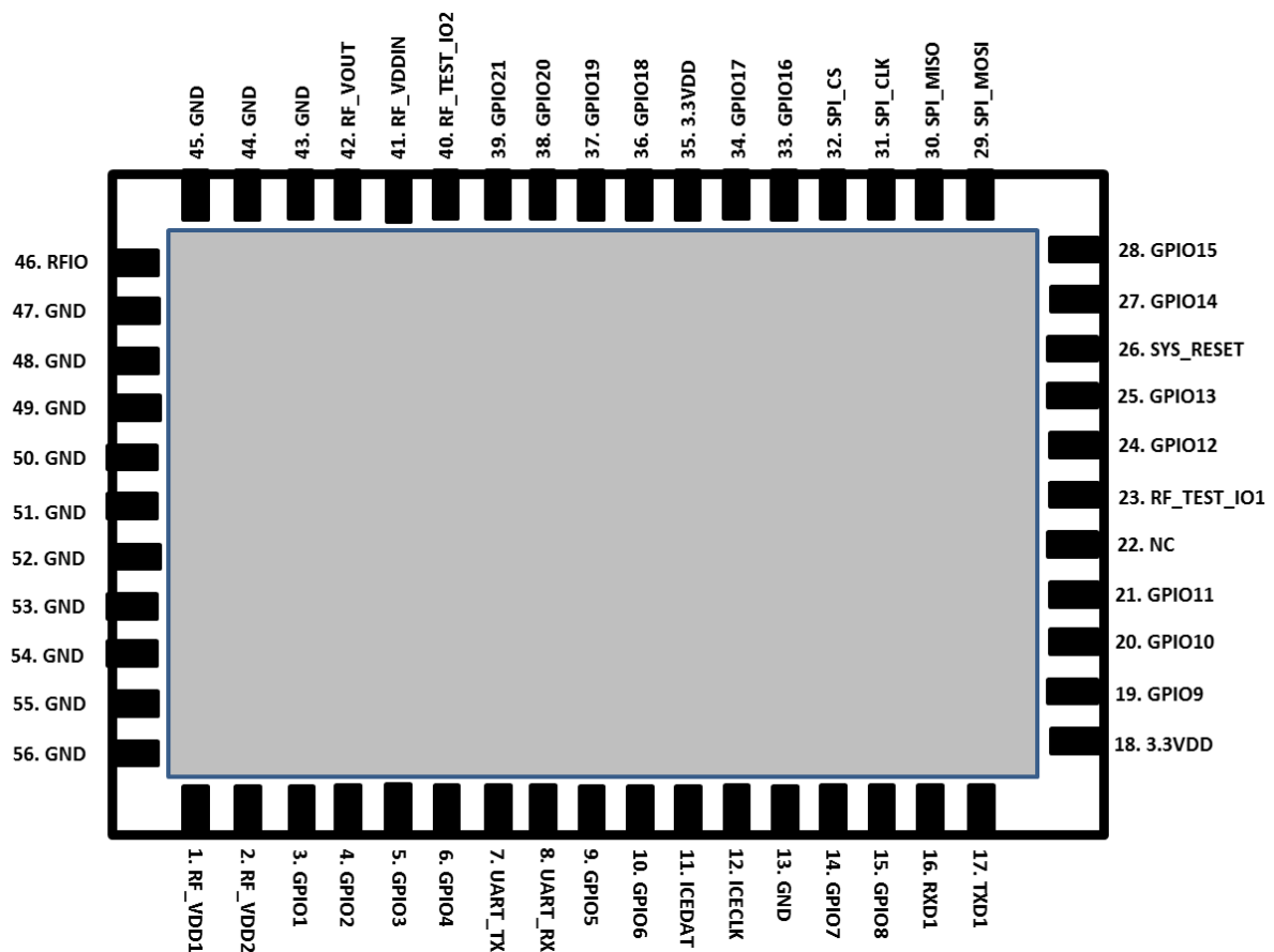
Figure4. Pin diagram
