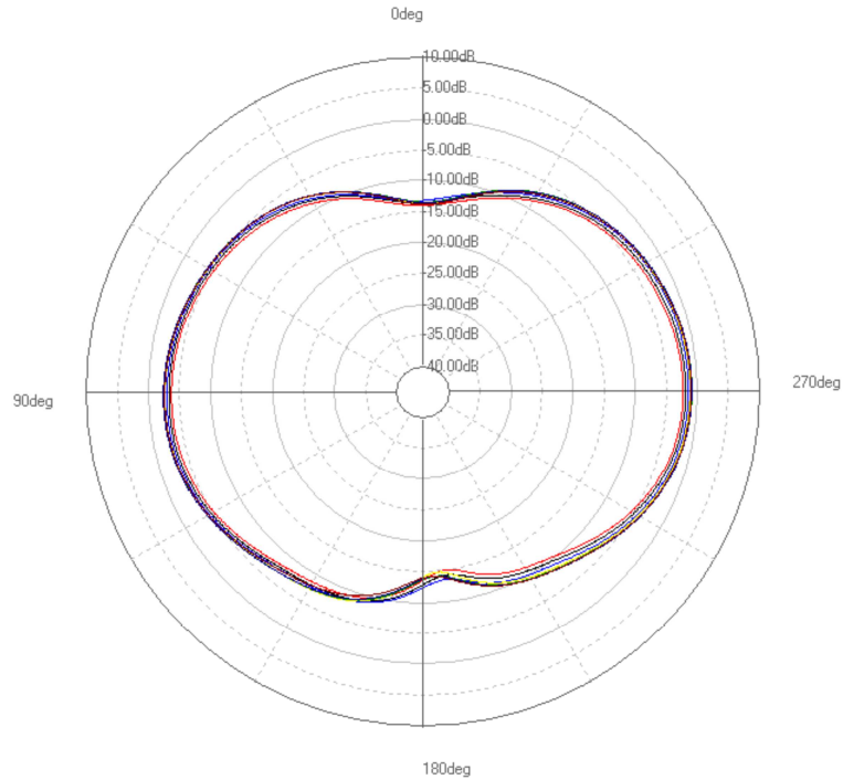
Y-Z Plane
