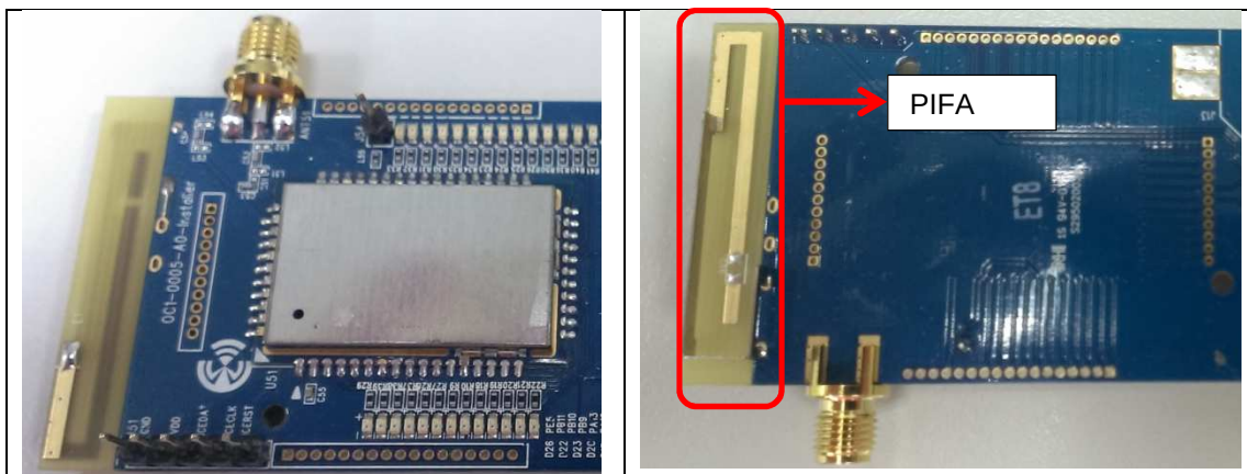
Figure16. PIFA antenna
