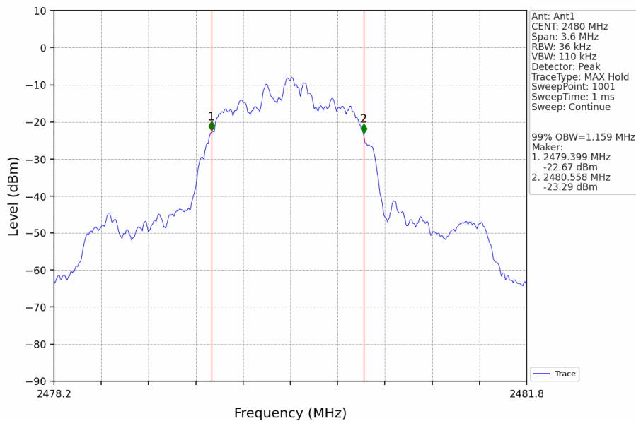
Pi/4DQPSK_2DH5_HCH_2480MHz_Ant1_NTNV
