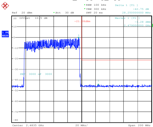
3DH1_Hopping_Upper
