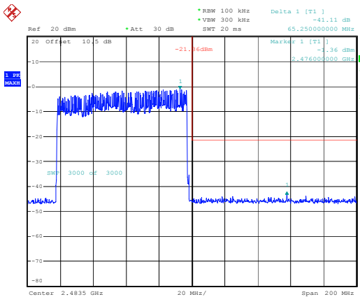
2DH1_Hopping_Upper
