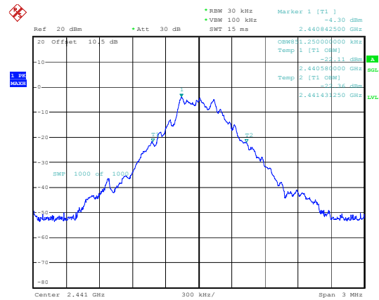
DH1_Middle
