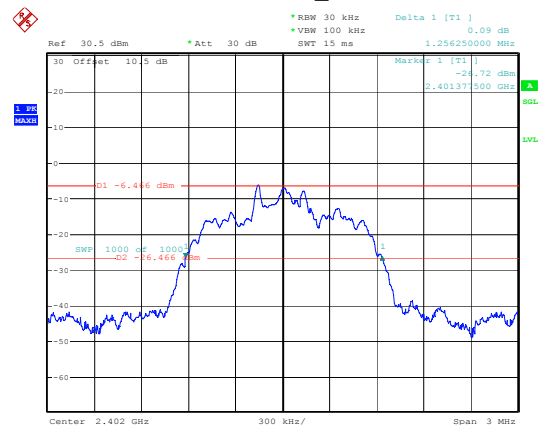
2DH1_Low
