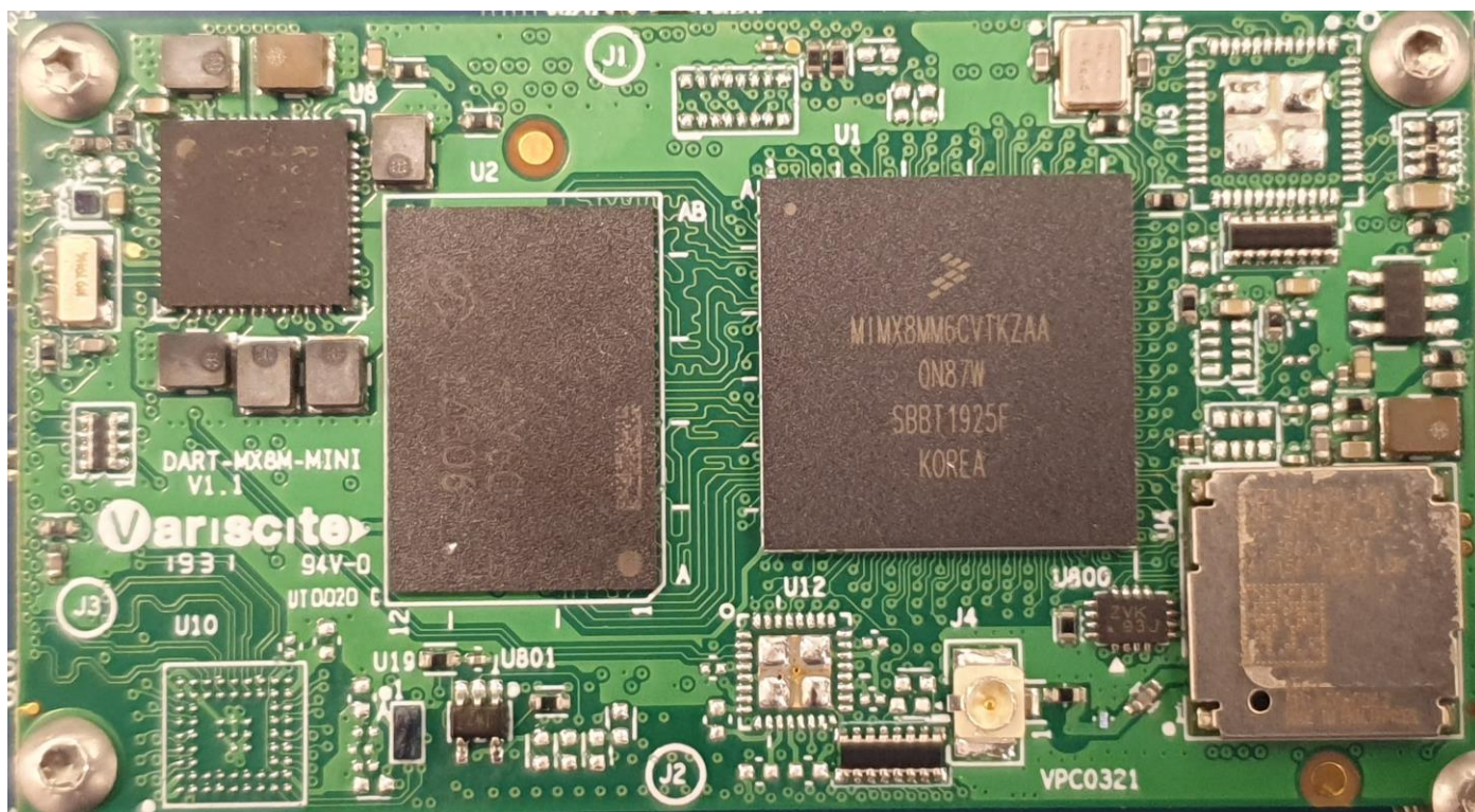
Figure 24 Top View CPU with the Sterling-LWB5
