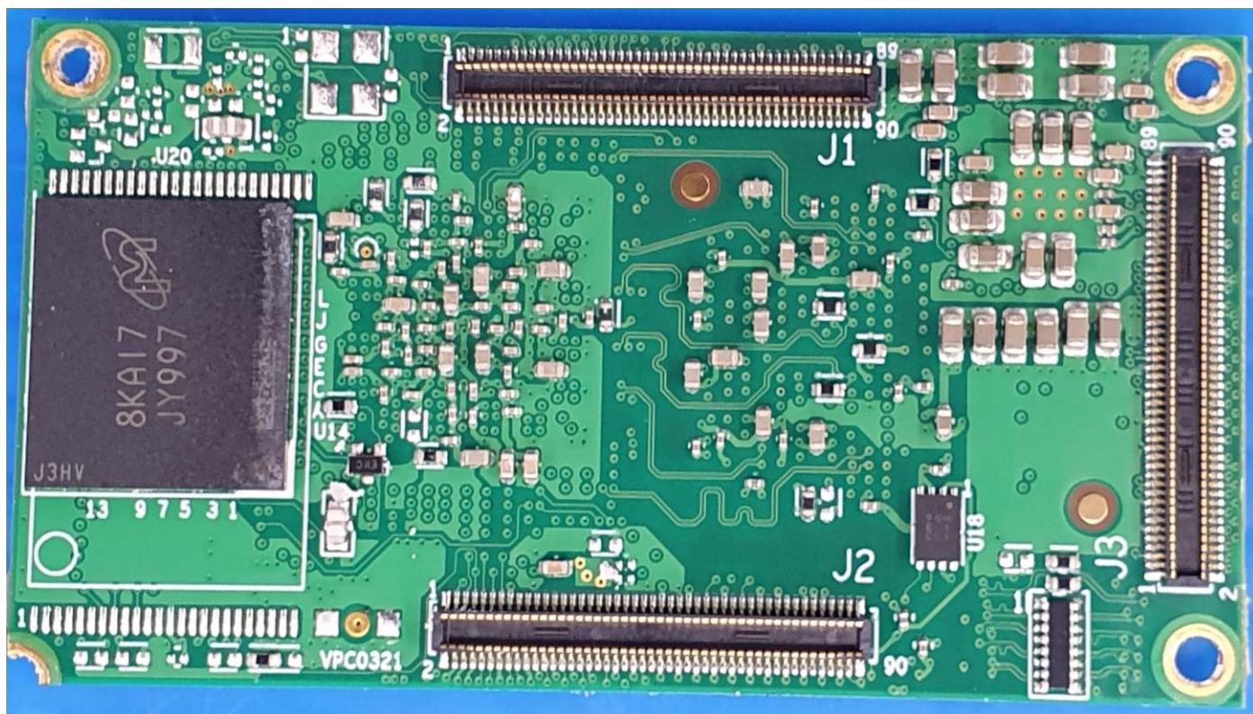
Figure 25 Bottom View CPU
