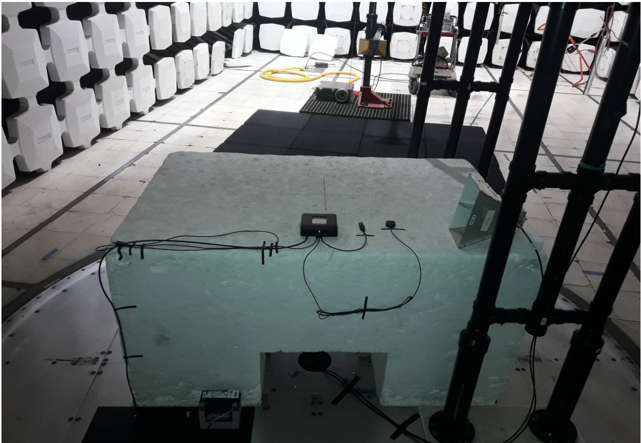
Test Configuration Photograph #3 (Radiated Emissions)
