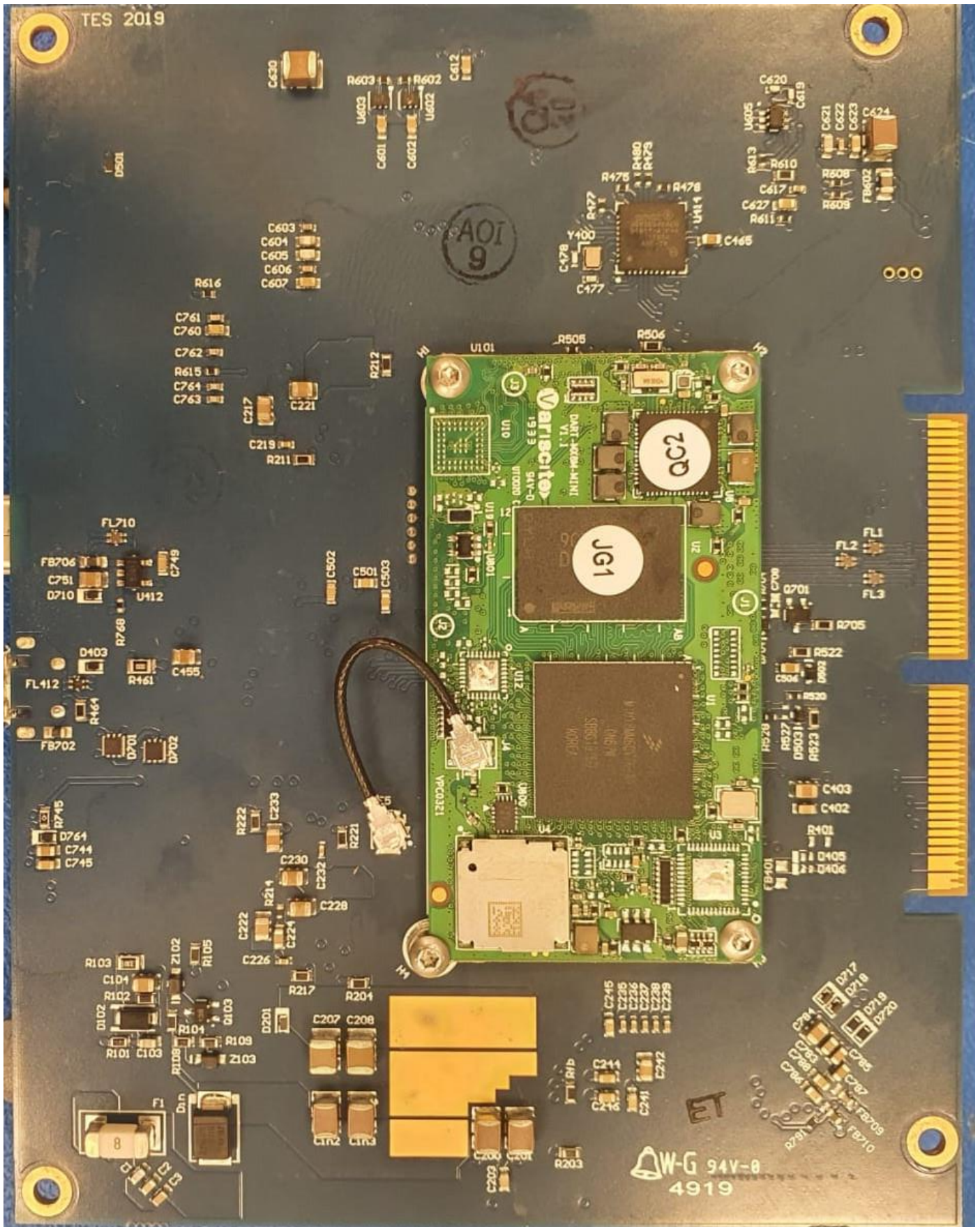
Figure 12 897602 PCBA, Carrier Board CPU AT&T PCB Bottom View
