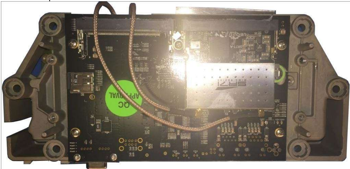
8. Internal Top 2
