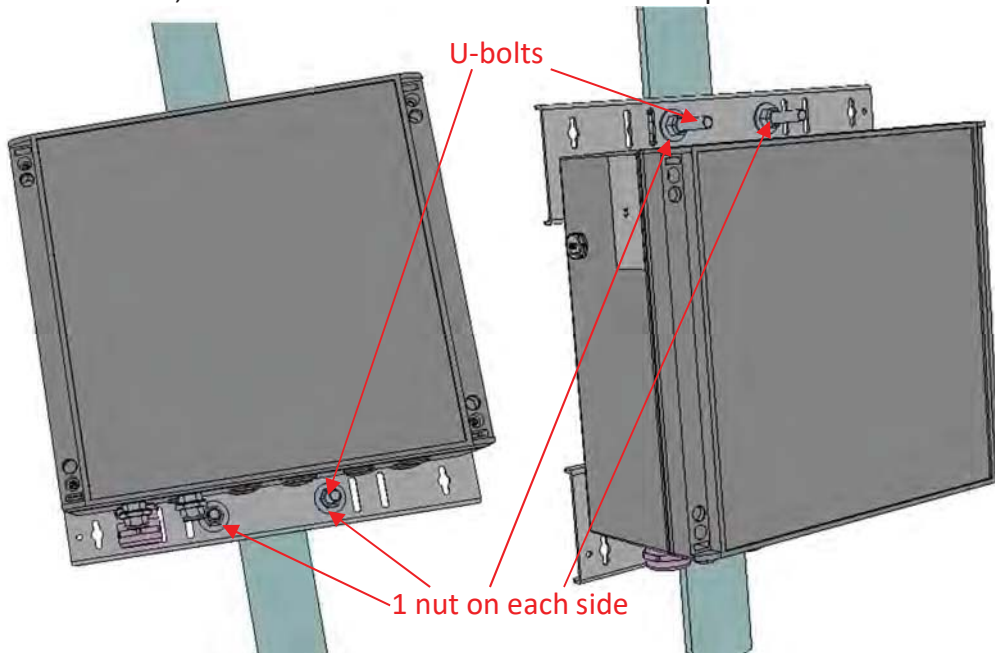
Figure 117 : Standard casing - Pole mount using U-bolts
