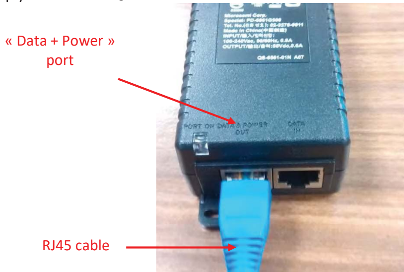
Figure 157 : Ethernet connection on PoE injector side
