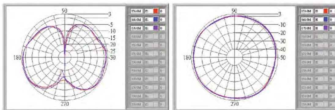
Figure 92 : Typical gain of 3dBi omnidirectional antenna
