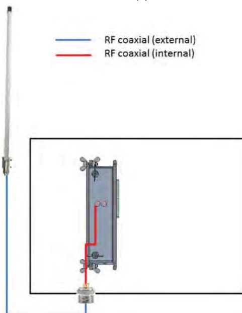
Figure 145 : Single LoRa module / single omnidirectional antenna connections
