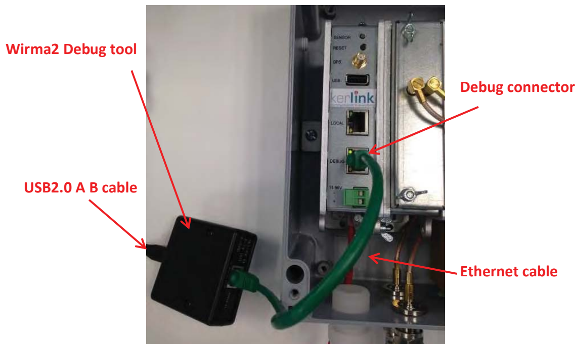
Figure 82 : WIRMA2 Debug Tool connected to the CPU module
