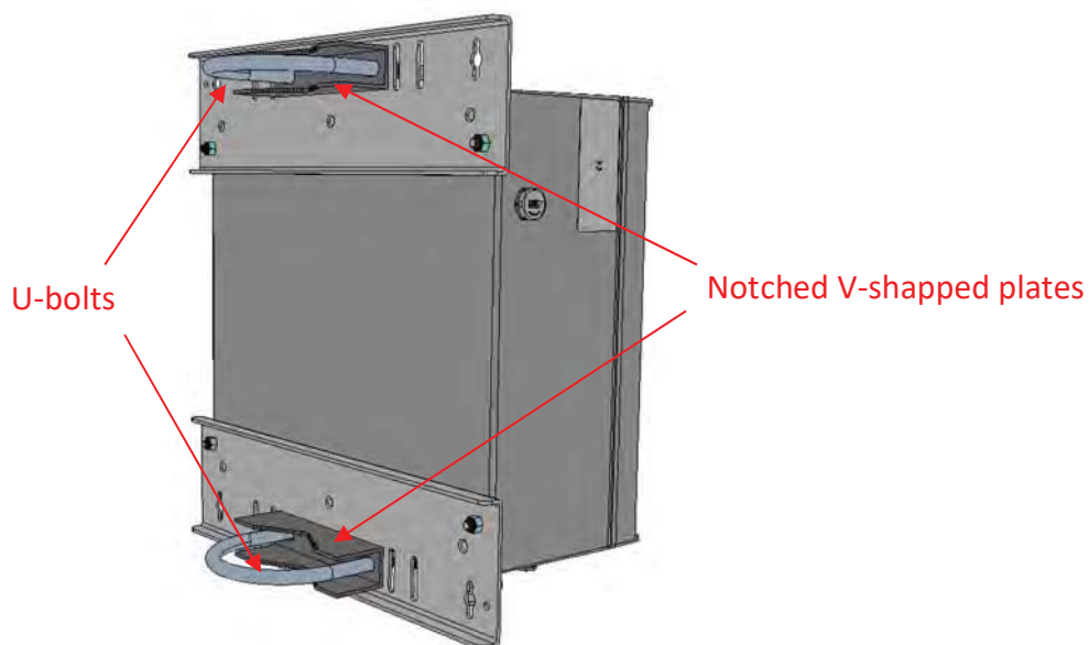
Figure 118 : Compact casing - rear view of the pole mounting using U-bolt (no pole represented)
