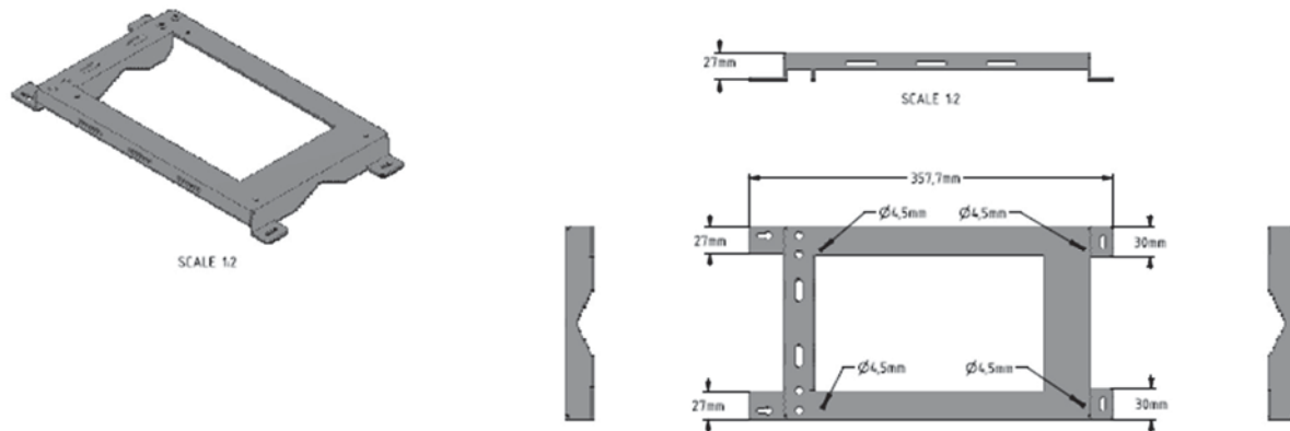
Figure 109 : Compact casing mounting kit dimensions
