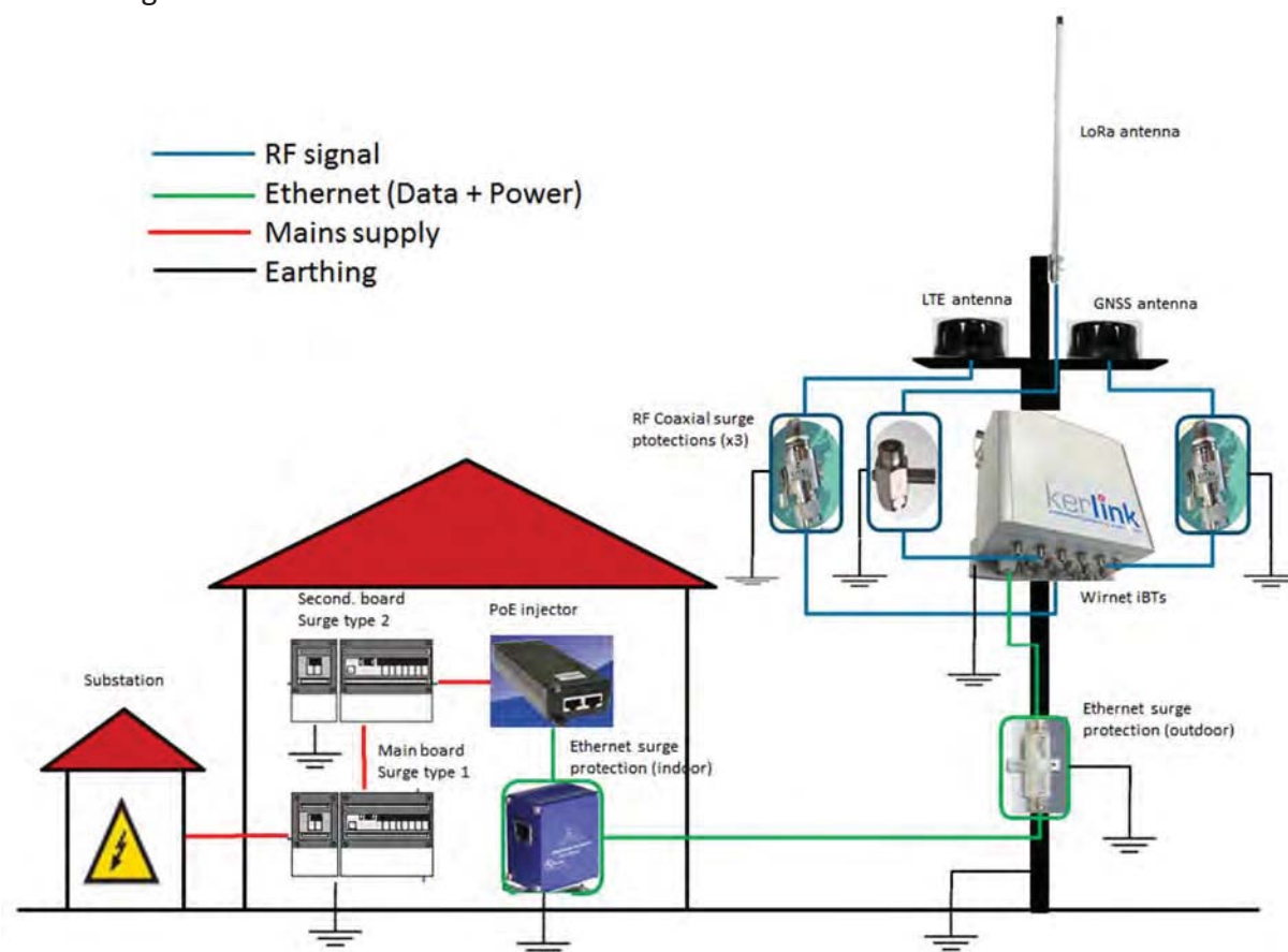
Figure 159 : Installation with recommended lighting protections
