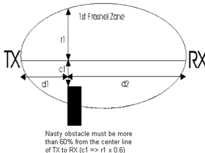
Figure 26 : Fresnel ellipsoid clearance
