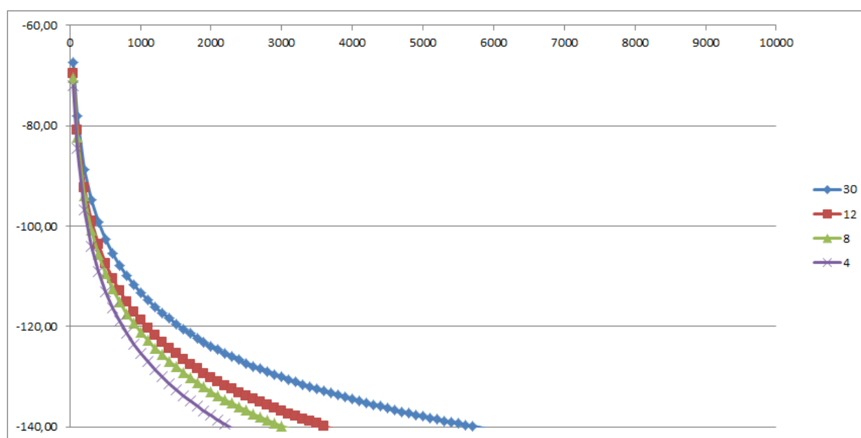
Figure 22 : Urban (small city) Hata propagation model vs height of the antenna
