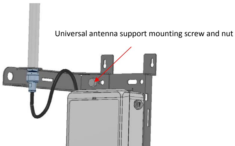
Figure 30 : attachment of the antenna on the mounting set
