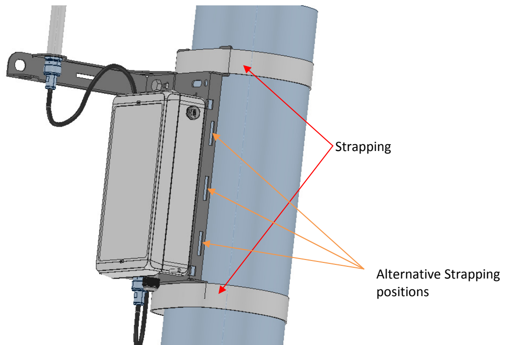
Figure 20 : Pole mount set using strapping
