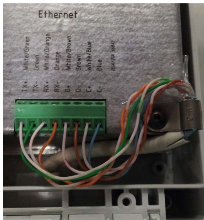
Figure 11 : Ethernet connection
