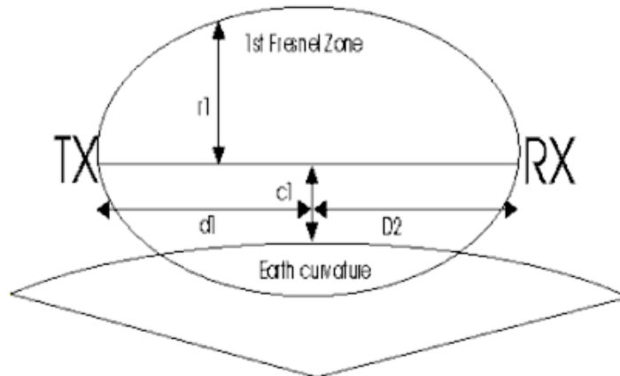
Figure 27 : Fresnel ellipsoid and earth curvature
