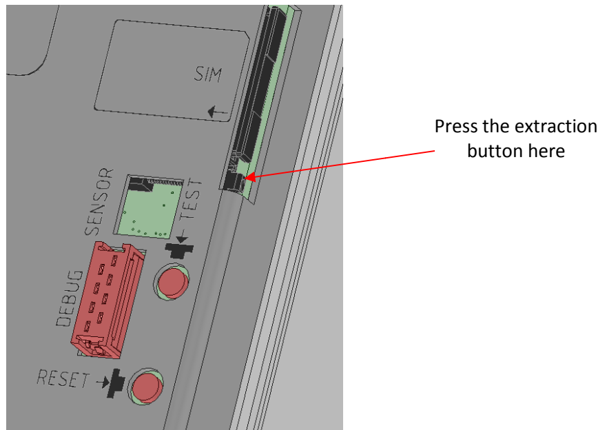
Figure 33 : SIM Card
