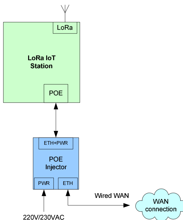
Figure 8 : Single station installation (No SIM)
