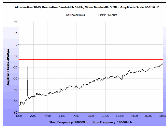
Plot 24. Radiated Spurious Emissions, High Channel, 1 GHz – 18 GHz, Part 24
