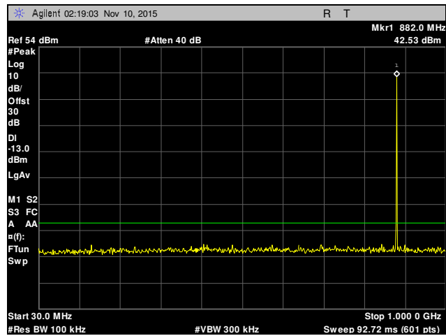
Plot 29. Conducted Spurious Emissions, Channel 190, 30 MHz – 1 GHz, Part 22
