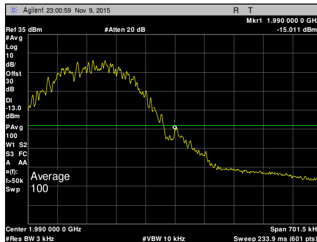
Plot 59. Conducted Band Edge, Channel 810, Part 24
