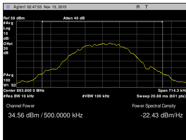
Plot 3, Channel 251, Conducted Power, Part 22
