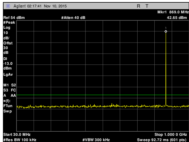
Plot 25. Conducted Spurious Emissions, Channel 128, 30 MHz – 1 GHz, Part 22
