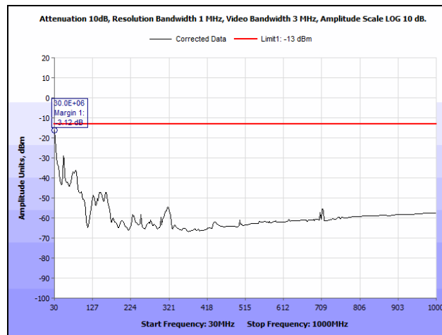
Plot 23. Radiated Spurious Emissions, High Channel, 30 MHz – 1 GHz, Part 24
