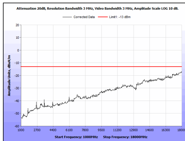
Plot 14. Radiated Spurious Emissions, Low Channel, 1 GHz – 18 GHz, Part 22
