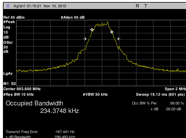
Plot 9. Occupied Bandwidth, Channel 251, Part 22
