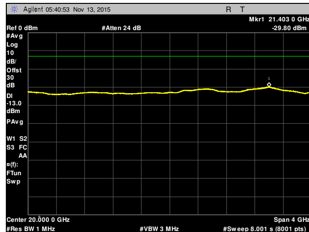
Plot 48. Conducted Spurious Emissions, Channel 661, 18 GHz – 22 GHz, Part 24
