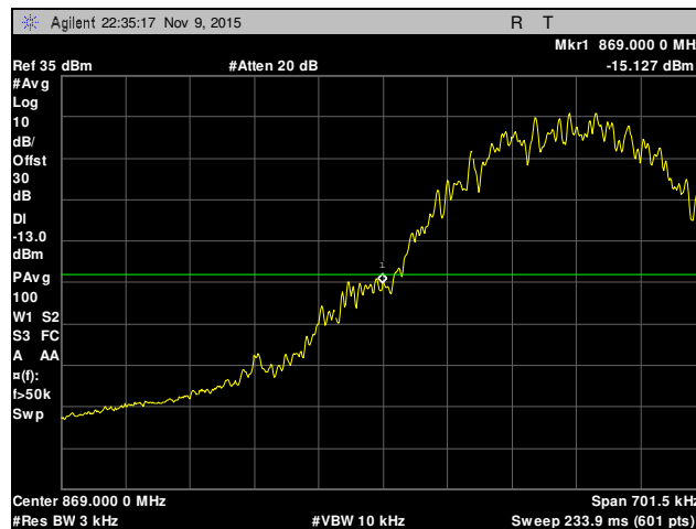
Plot 56. Conducted Band Edge, Channel 128, Part 22
