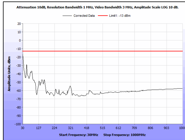
Plot 19. Radiated Spurious Emissions, Low Channel, 30 MHz – 1 GHz, Part 24
