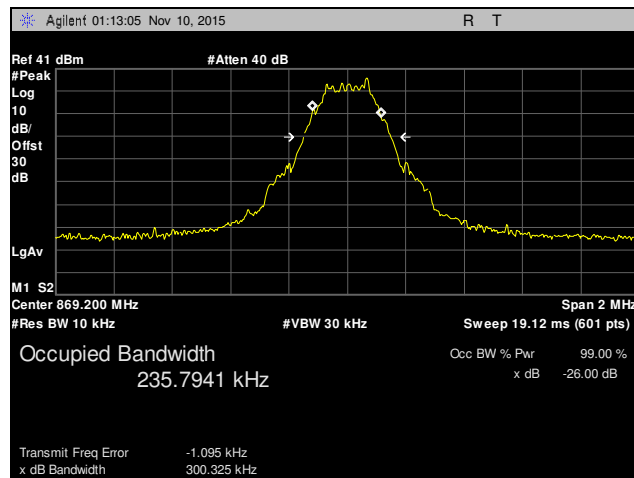
Plot 7. Occupied Bandwidth, Channel 128, Part 22
