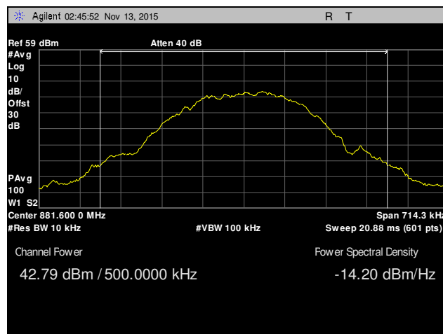
Plot 2, Channel 190, Conducted Power, Part 22
