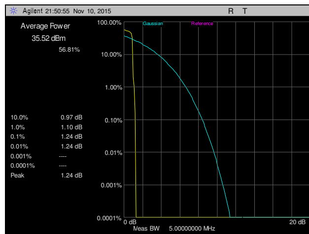
Plot 61. Peak to Average Ratio, Channel 190, Part 22
