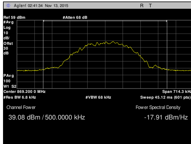
Plot 1, Channel 128, Conducted Power, Part 22
