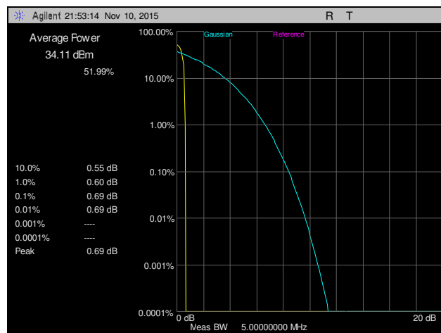
Plot 62. Peak to Average Ratio, Channel 251, Part 22
