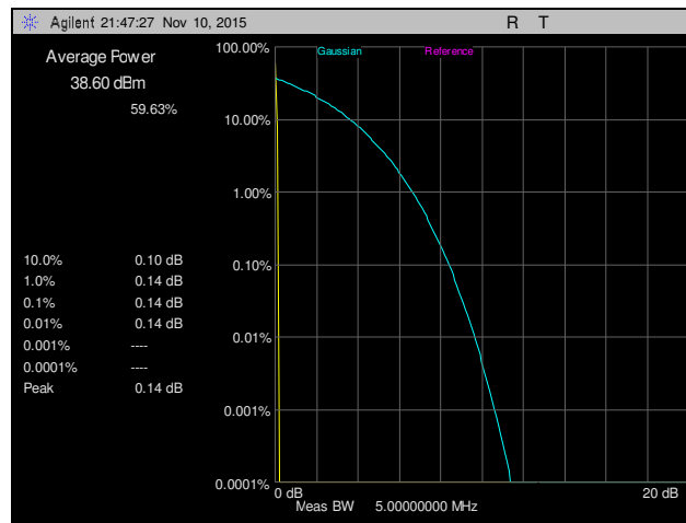
Plot 60. Peak to Average Ratio, Channel 128, Part 22
