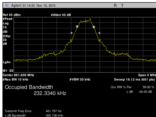
Plot 8. Occupied Bandwidth, Channel 190, Part 22
