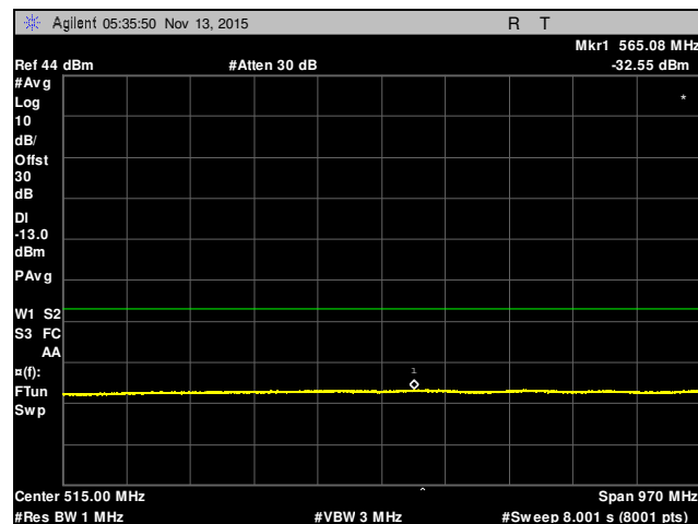
Plot 42. Conducted Spurious Emissions, Channel 661, 30 MHz – 1 GHz, Part 24
