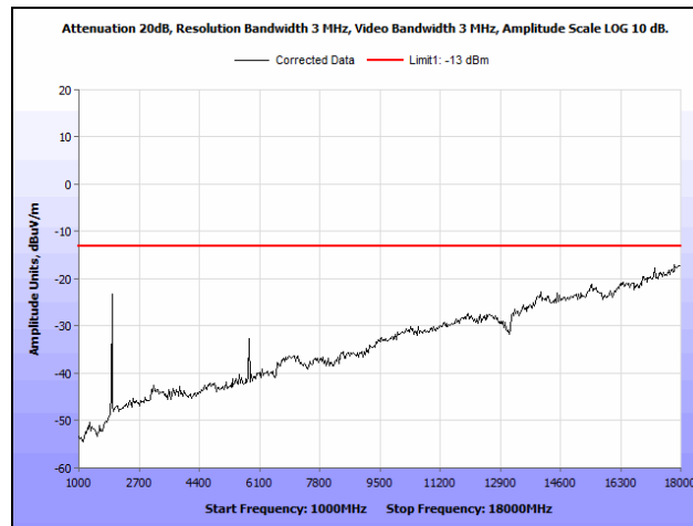
Plot 22. Radiated Spurious Emissions, Mid Channel, 1 GHz – 18 GHz, Part 24
