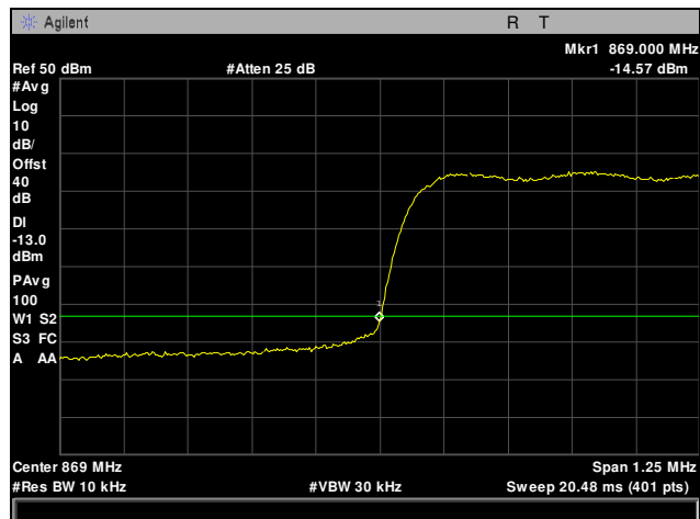
Plot 93. Conducted Band Edge, Channel 1013, Part 22
