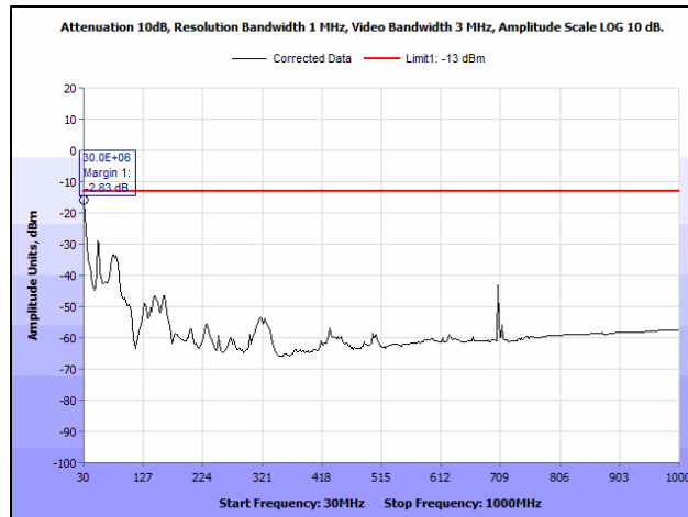
Plot 93. Radiated Spurious Emissions, Mid Channel, 30 MHz – 1 GHz, Part 27, 10 MHz, LTE2100
