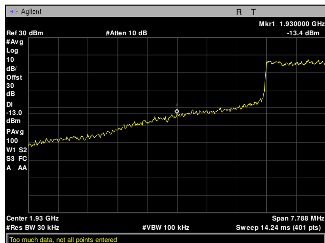
Plot 249. Conducted Band Edge, Channel 646 (Full Power), 5 MHz, Part 24
