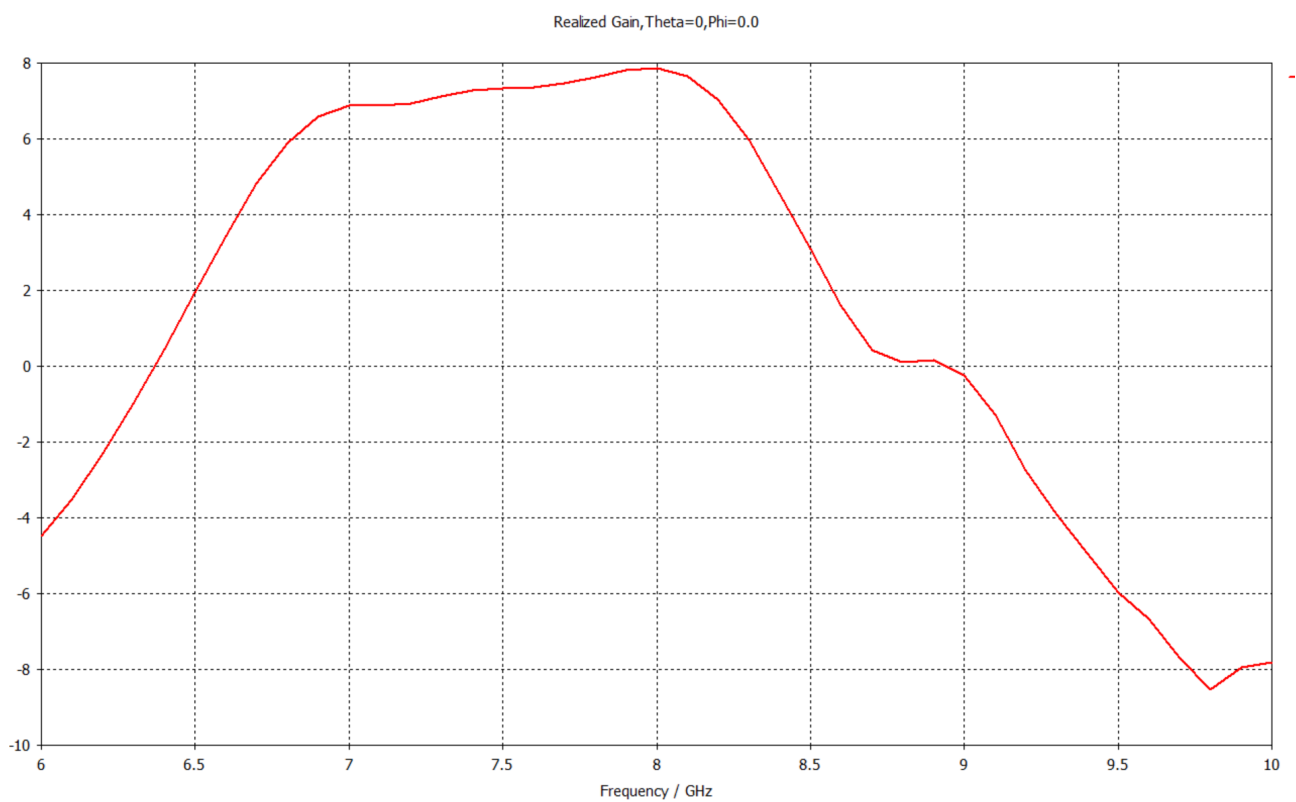
3 Antenna Gain Over Frequency
