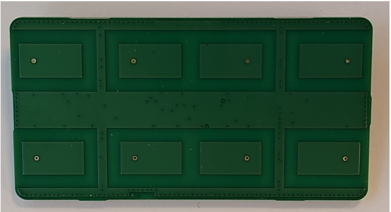
2 Antenna side
