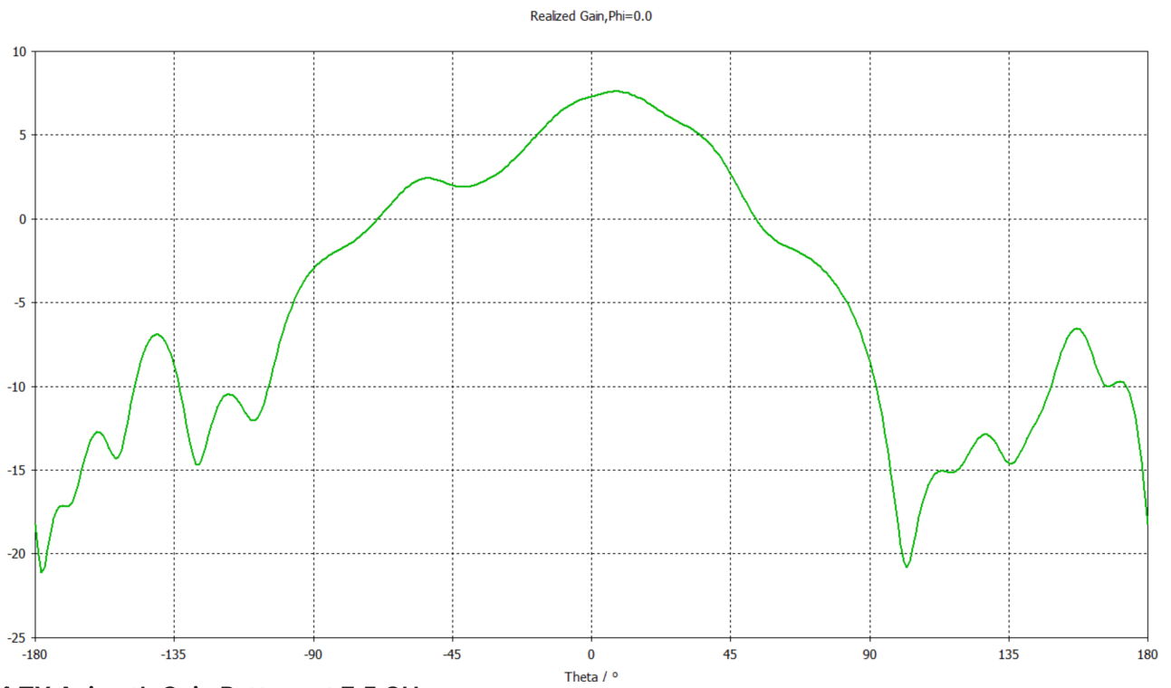
4 TX Azimuth Gain Pattern at 7.5 GHz
