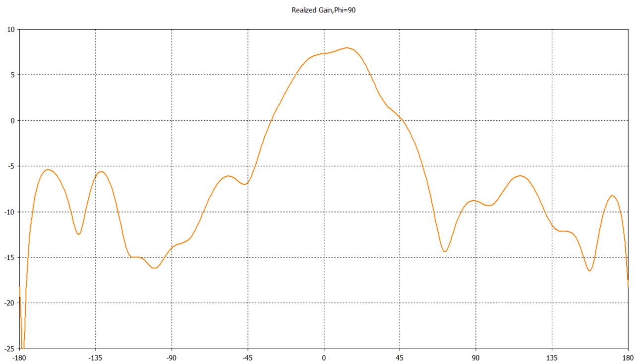
5 TX Elevation Gain Pattern at 7.5 GHz
