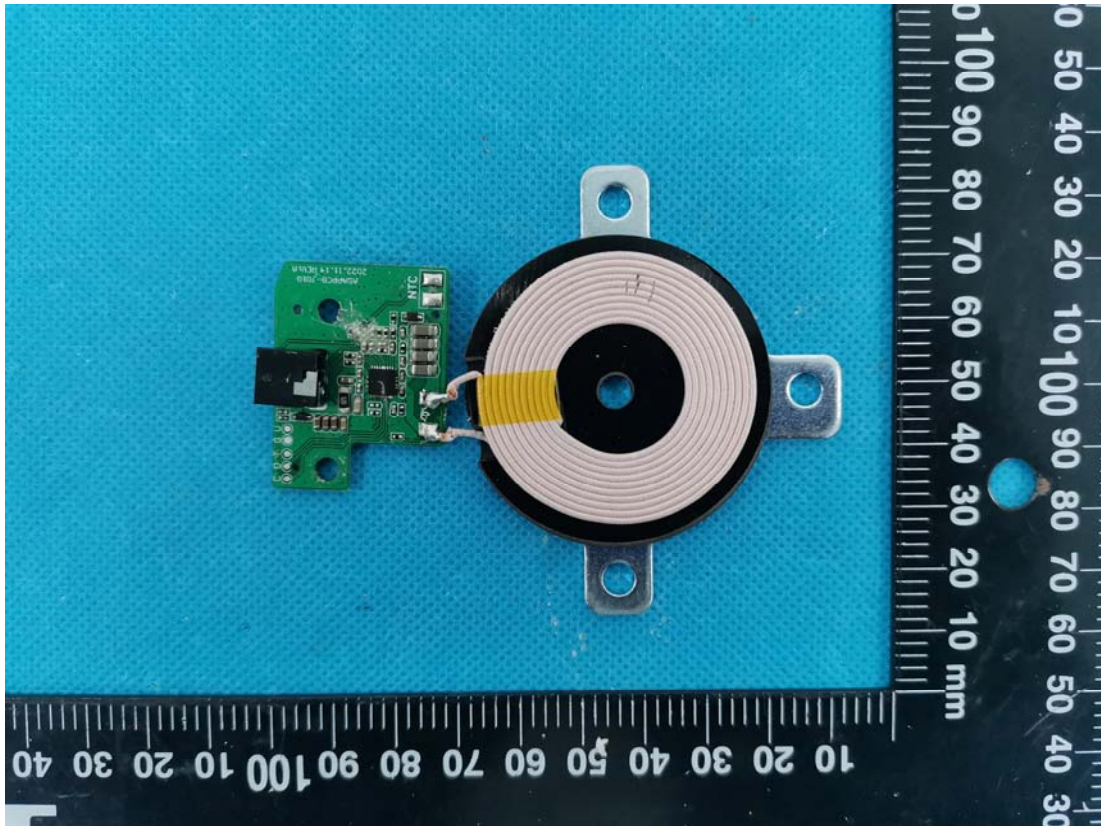
Coil
