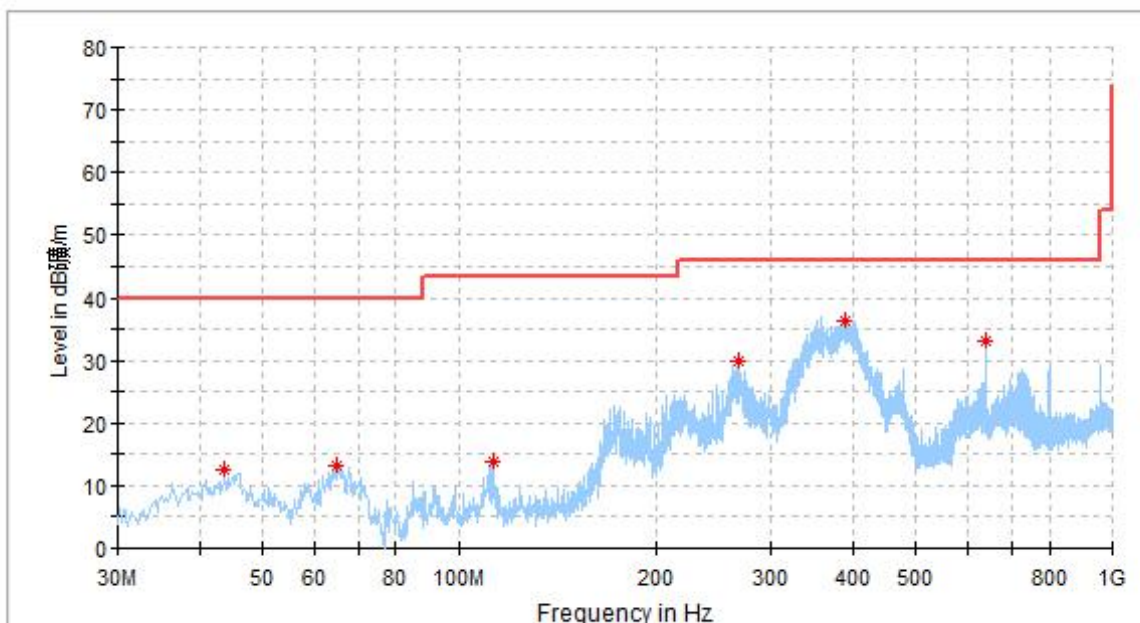
(802.11b_2437MHz, Antenna Horizontal, 30MHz to 1GHz)
