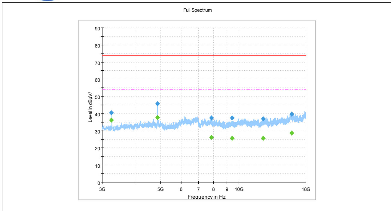
(802.11b_2437MHz, Antenna Horizontal, 3GHz to 18GHz)
