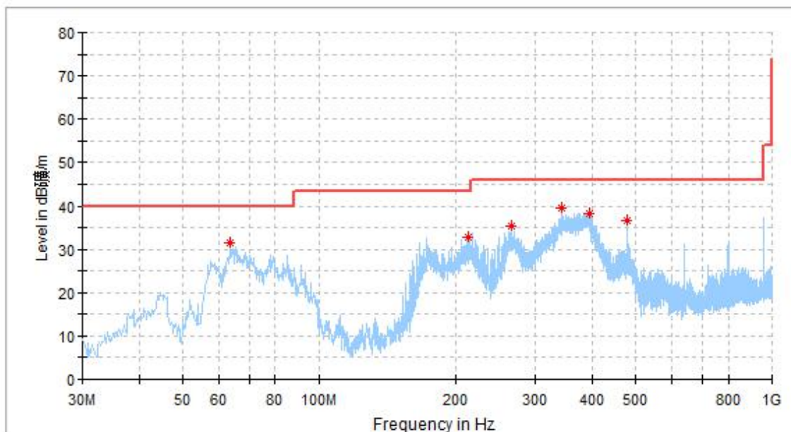
(802.11b_2437MHz, Antenna Vertical, 30MHz to 1GHz)
