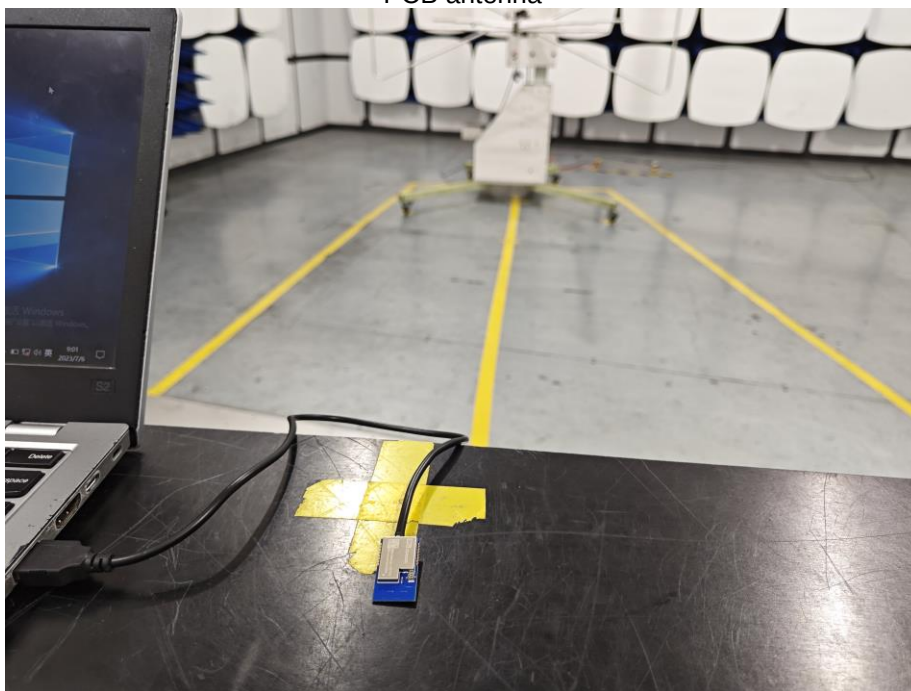
PCB antenna
