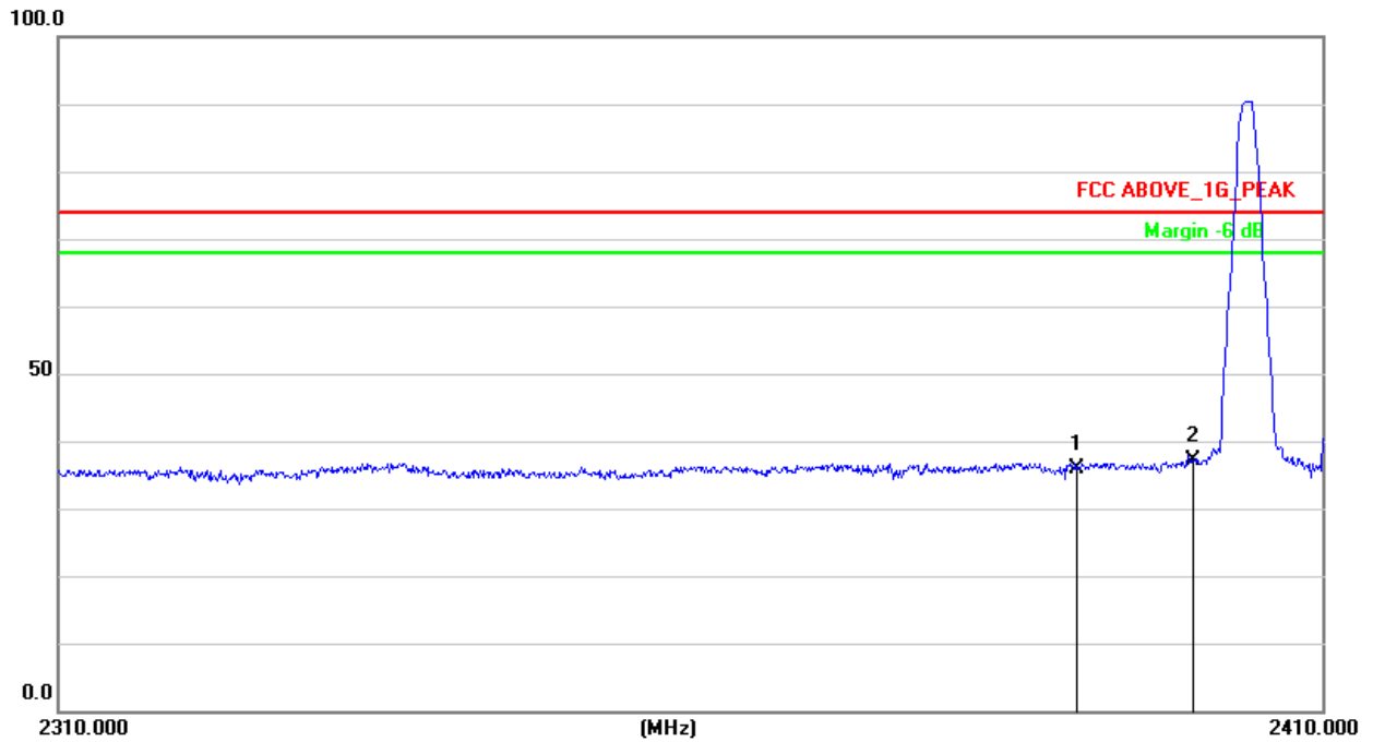
2404 MHz Horizontal
