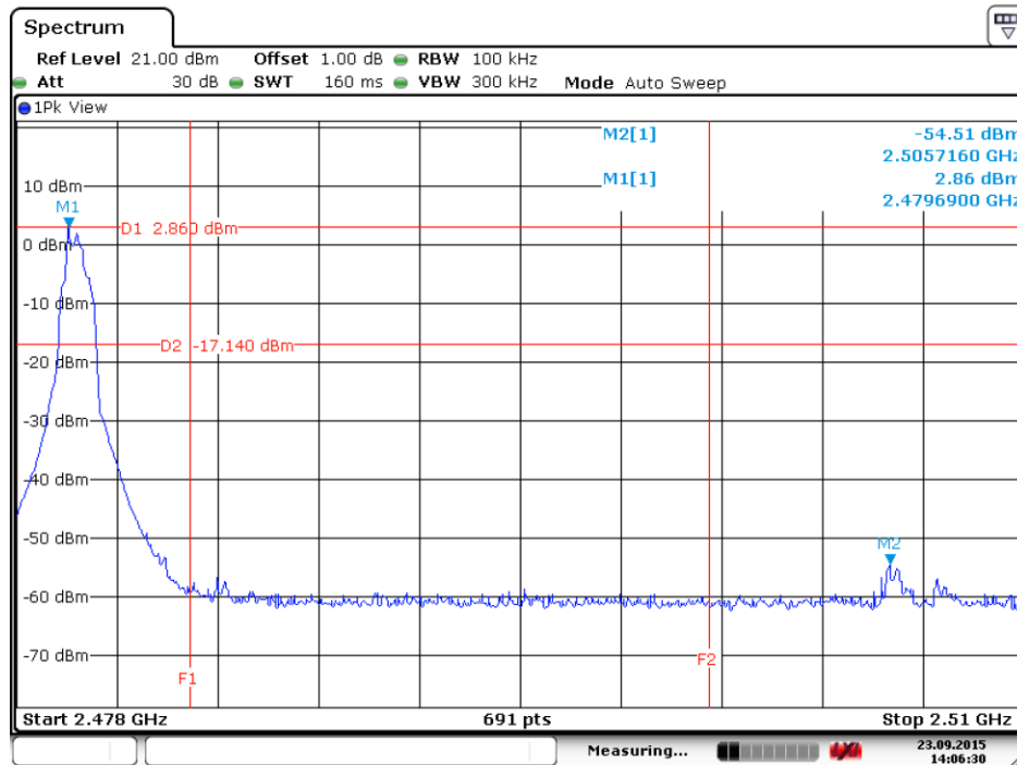
High Band Edge Plot on Channel 39
