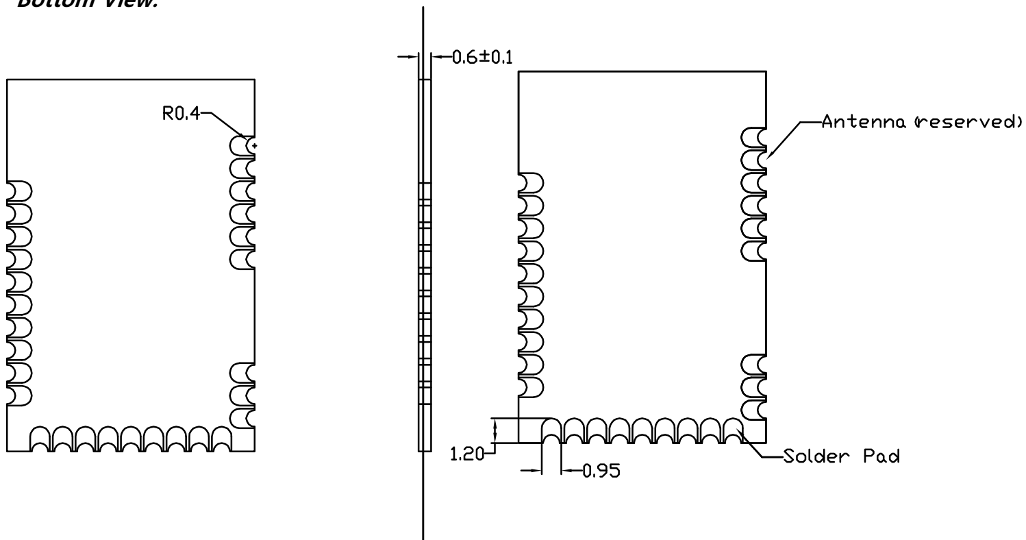
Bottom View:
