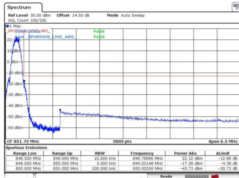
Higher Band Edge Plot on Channel 251 (848.8 MHz)
