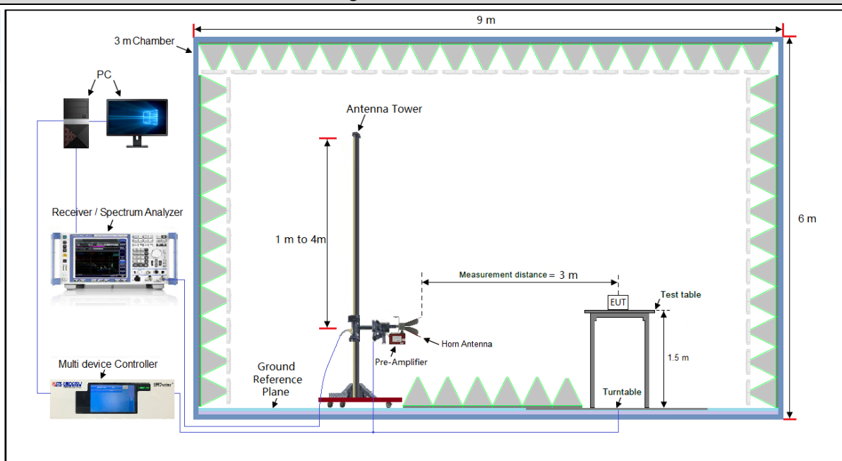
Figure 3. Above 1GHz
