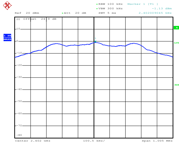
PSD 100kHz Plot on Channel 00
