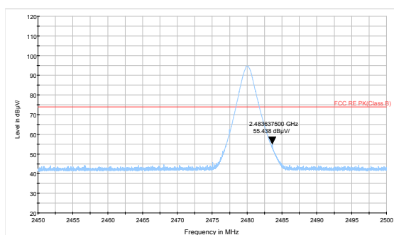
3DH5-Channel 78: Peak
