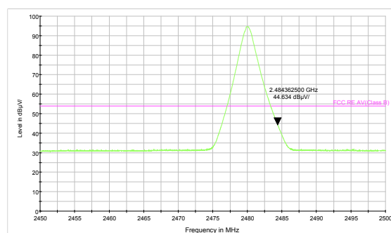
3DH5-Channel 78: Average
