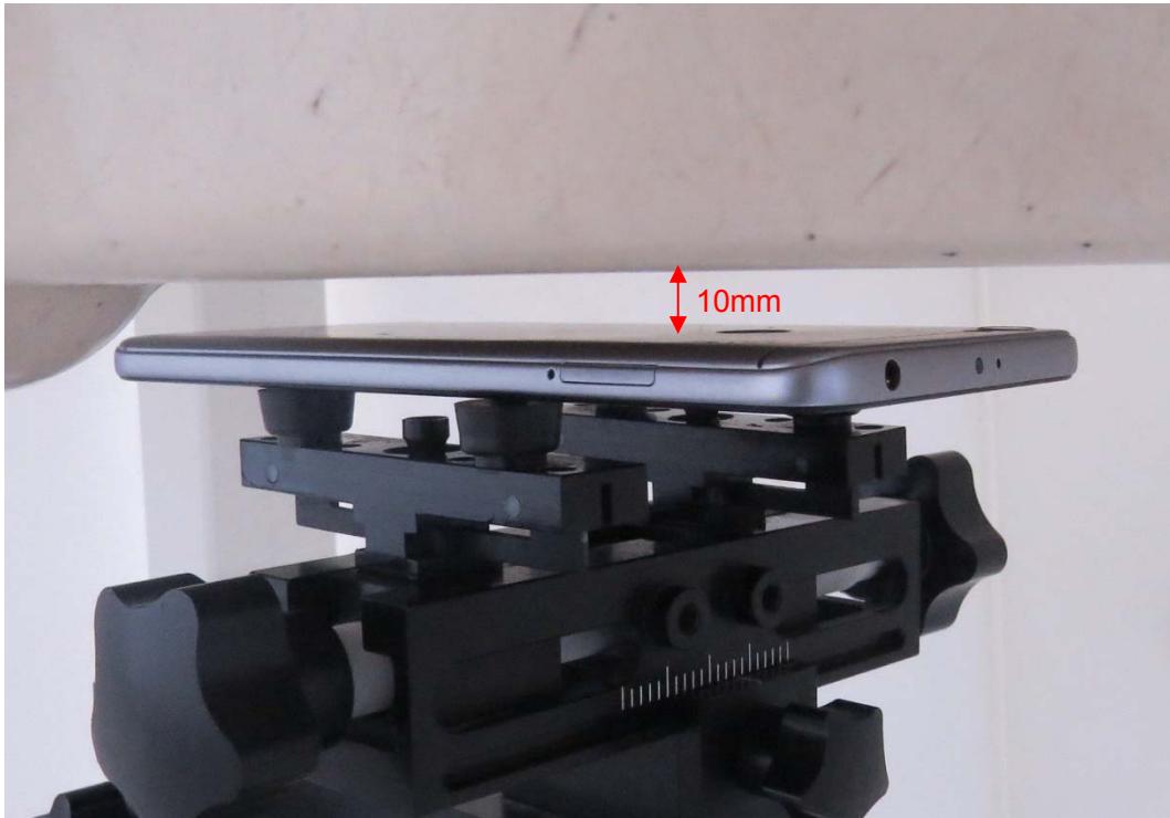
Picture 18: Back Side, the distance from handset to the bottom of the Phantom is 10mm
