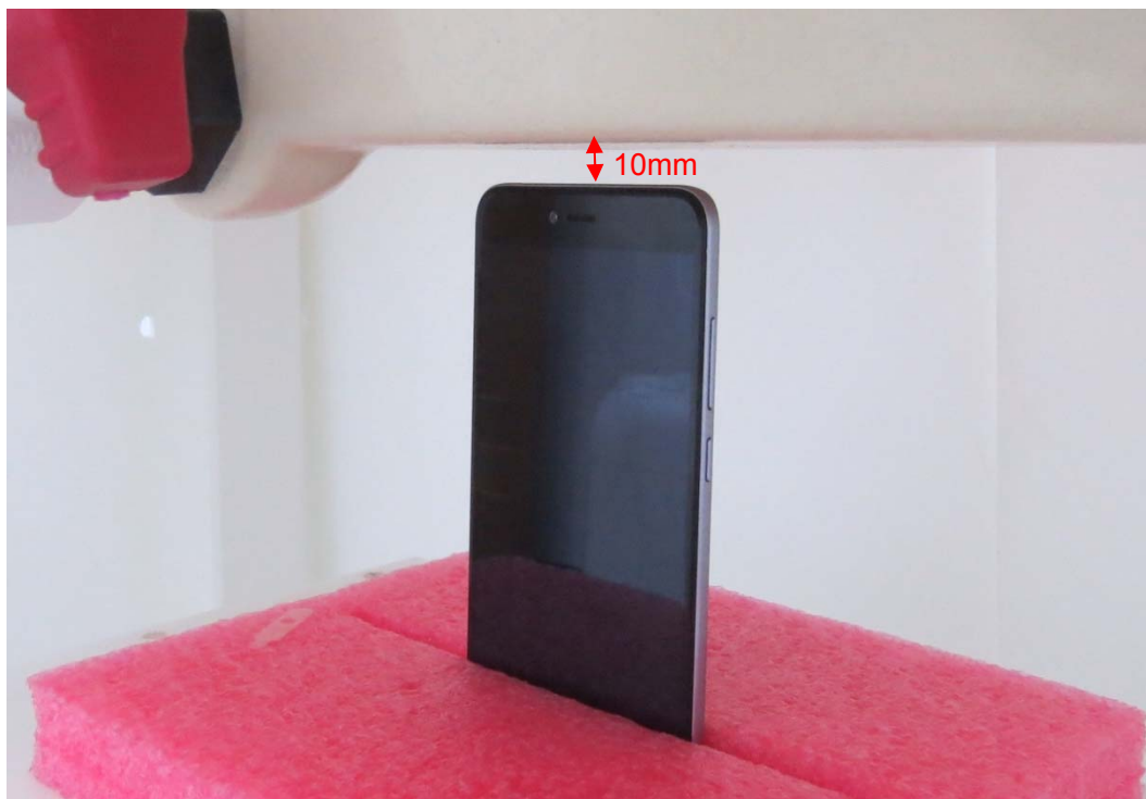
Picture 22: Top Side, the distance from handset to the bottom of the Phantom is 10mm
