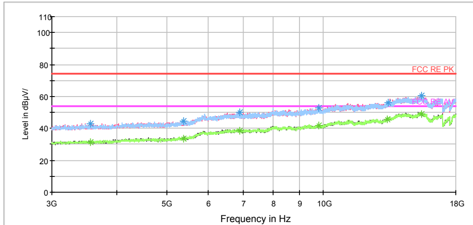
Radiates Emission from 3GHz to 18GHz
