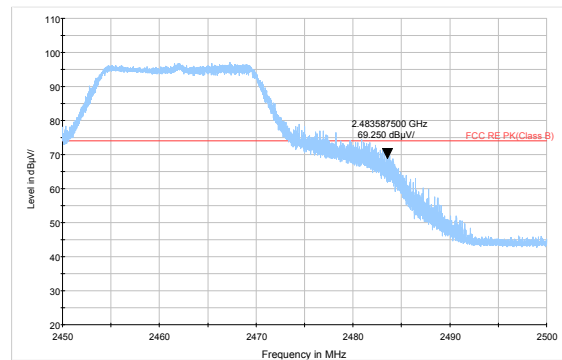
802.11g-Channel 11: Peak
