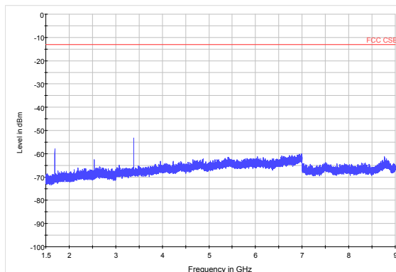
LTE Band 5 10MHz CH-Low 1.5GHz~9GHz
