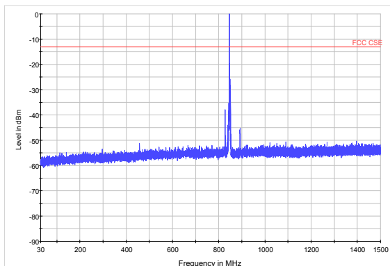
LTE Band 5 10MHz CH-Low 30MHz~1.5GHz
