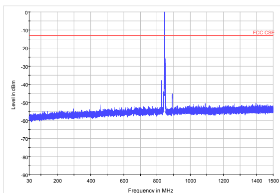
LTE Band 5 5MHz CH-Low 30MHz~1.5GHz
