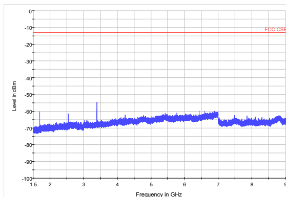
LTE Band 5 3MHz CH-Low 1.5GHz~9GHz
