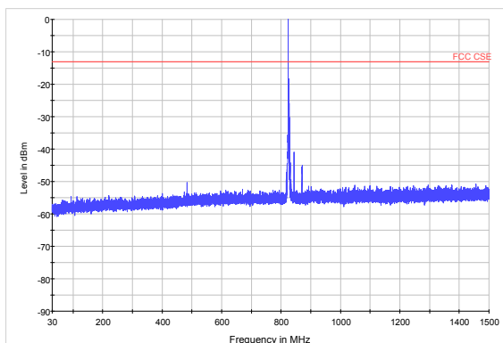
LTE Band 5 3MHz CH-Low 30MHz~1.5GHz
