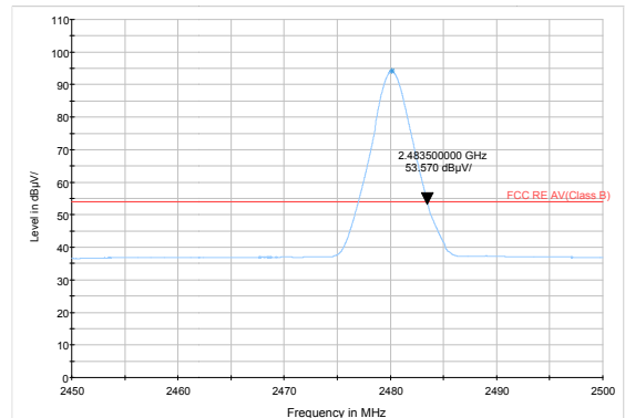
3DH5-Channel 78: Average
