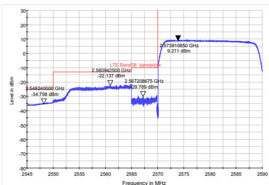
LTE Band 38 QPSK 20MHz CH-Low, RB 100
