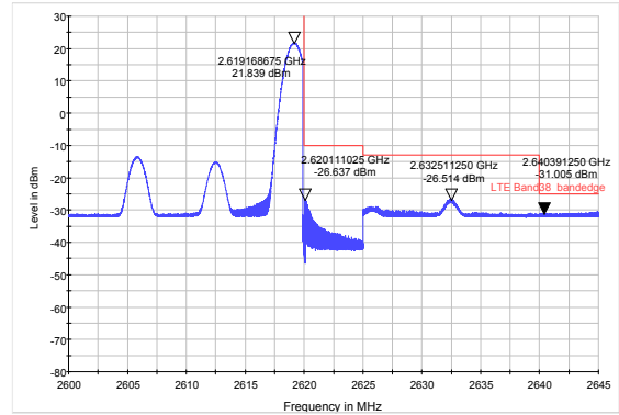
LTE Band 38 QPSK 15MHz CH-High, RB 1
