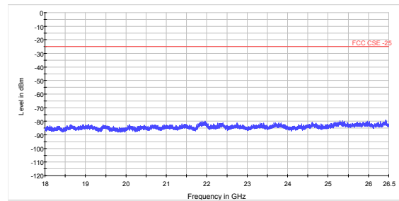
LTE Band 38 20MHz CH-Low 18GHz~26.5GHz
