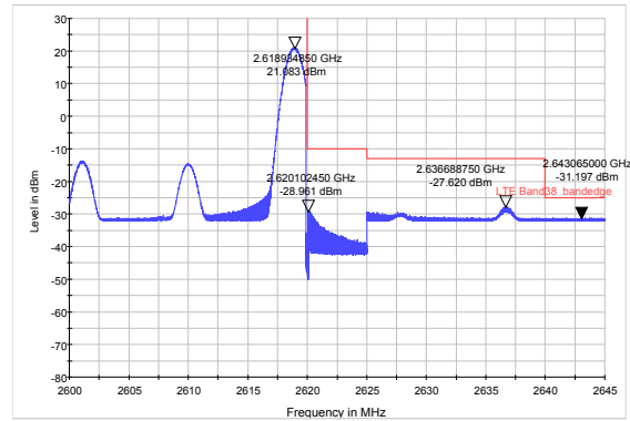
LTE Band 38 16QAM 20MHz CH-High, RB 100
