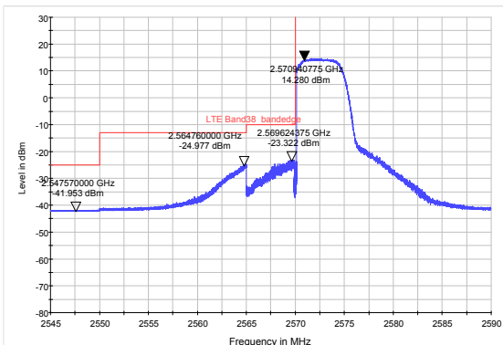
LTE Band 38 16QAM 10MHz CH-Low, RB 1
