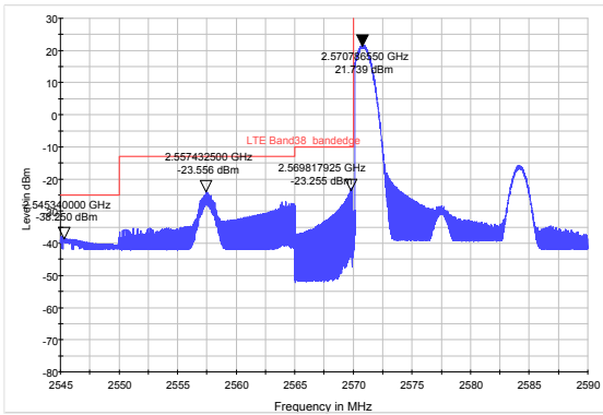
LTE Band 38 16QAM 15MHz CH-Low, RB 75
