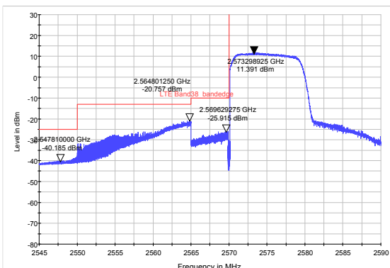
LTE Band 38 16QAM 10MHz CH-Low, RB 50
