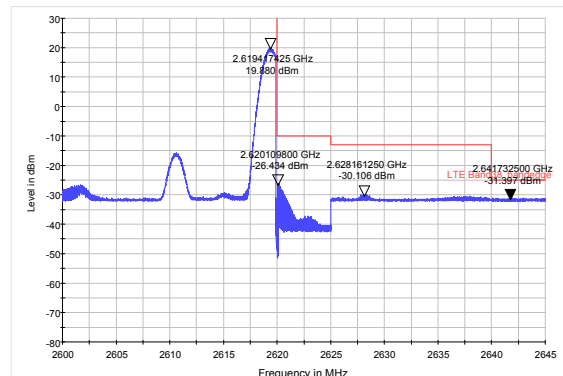
LTE Band 38 16QAM 10MHz CH-High, RB 50
