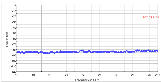
LTE Band 38 20MHz CH-Middle 18GHz~26.5GHz
