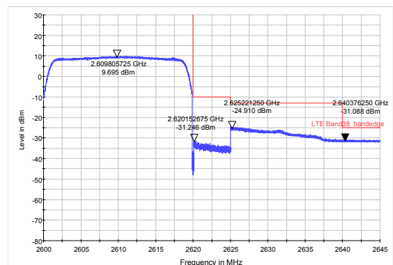
LTE Band 38 QPSK 20MHz CH-High, RB 100
