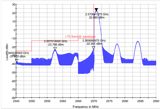
LTE Band 38 QPSK 15MHz CH-Low, RB 1
