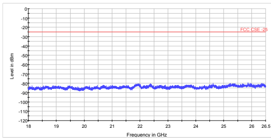
LTE Band 38 15MHz CH-Low 18GHz~26.5GHz
