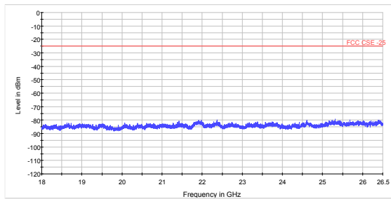
LTE Band 38 15MHz CH-High 18GHz~26.5GHz
