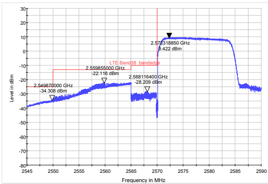
LTE Band 38 16QAM 20MHz CH-Low, RB 1
