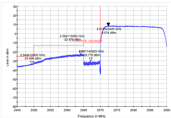
LTE Band 38 16QAM 20MHz CH-Low, RB 100
