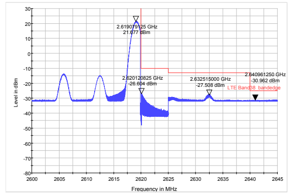
LTE Band 38 16QAM 15MHz CH-High, RB 75
