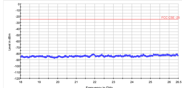
LTE Band 38 15MHz CH-Middle 18GHz~26.5GHz
