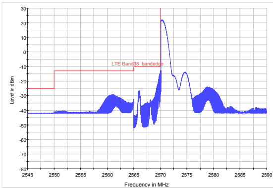
LTE Band 38 16QAM 5MHz CH-Low, RB 25
