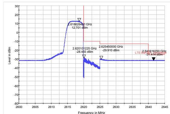
LTE Band 38 16QAM 10MHz CH-High, RB 1
