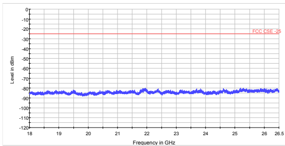
LTE Band 38 5MHz CH-Low 18GHz~26.5GHz
