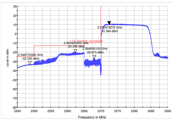
LTE Band 38 QPSK 20MHz CH-Low, RB 1
