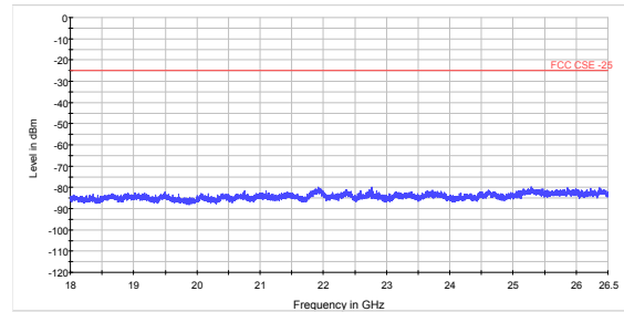
LTE Band 7 10MHz CH-High 18GHz~26.5GHz
