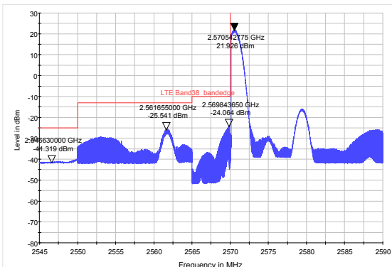
LTE Band 38 16QAM 10MHz CH-Low, RB 50
