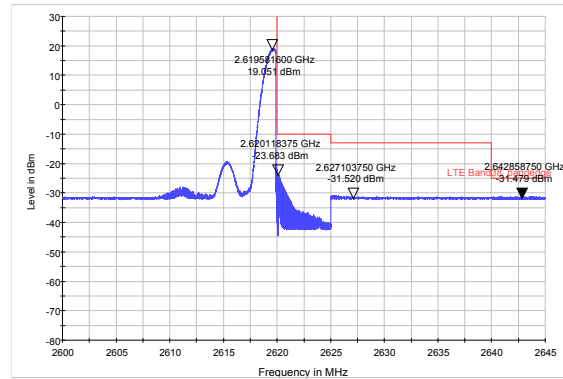
LTE Band 38 16QAM 5MHz CH-High, RB 25
