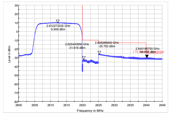
LTE Band 38 16QAM 20MHz CH-High, RB 1
