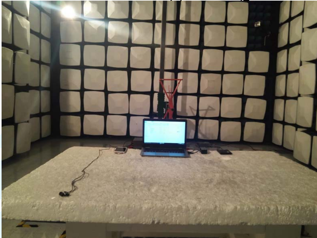
Radiated emission Test Setup (Below 1GHz) Mode 4
