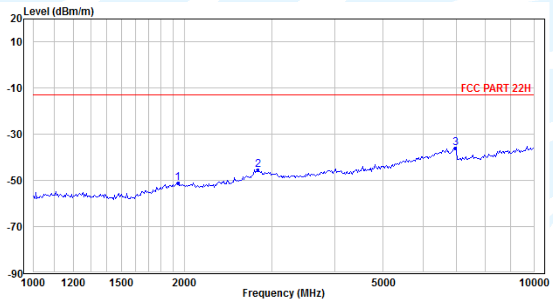
LTE Band 5; Bandwidth 3.0 MHz; Modulation: QPSK; RB: 1; 20525/836.5MHz _Vertical
