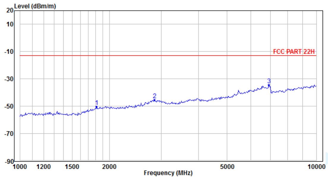
LTE Band 5; Bandwidth 3.0 MHz; Modulation: QPSK; RB: 1; 20525/836.5MHz _Horizontal
