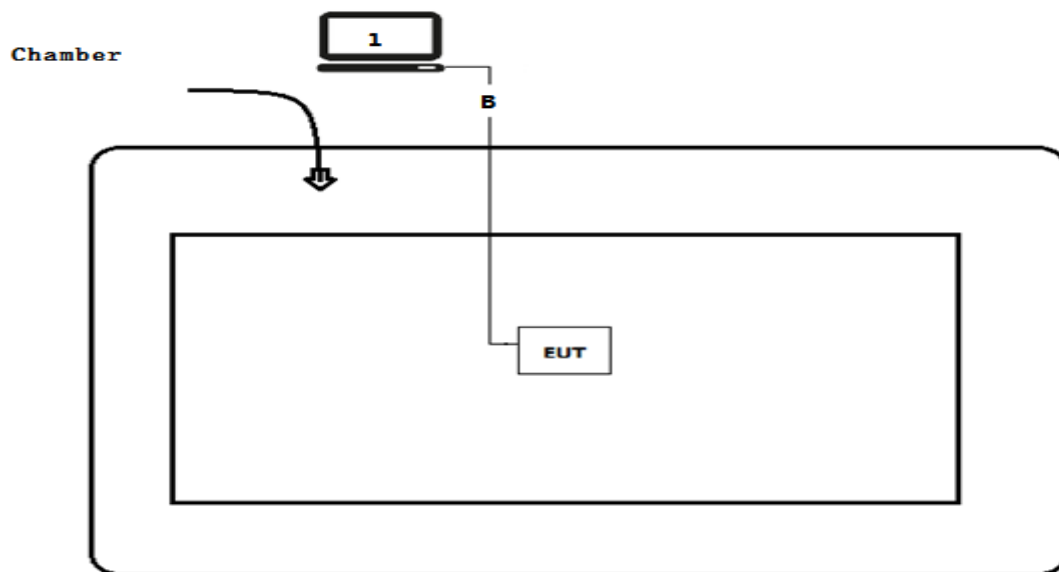
Test setup Diagram- Radiated Emission
