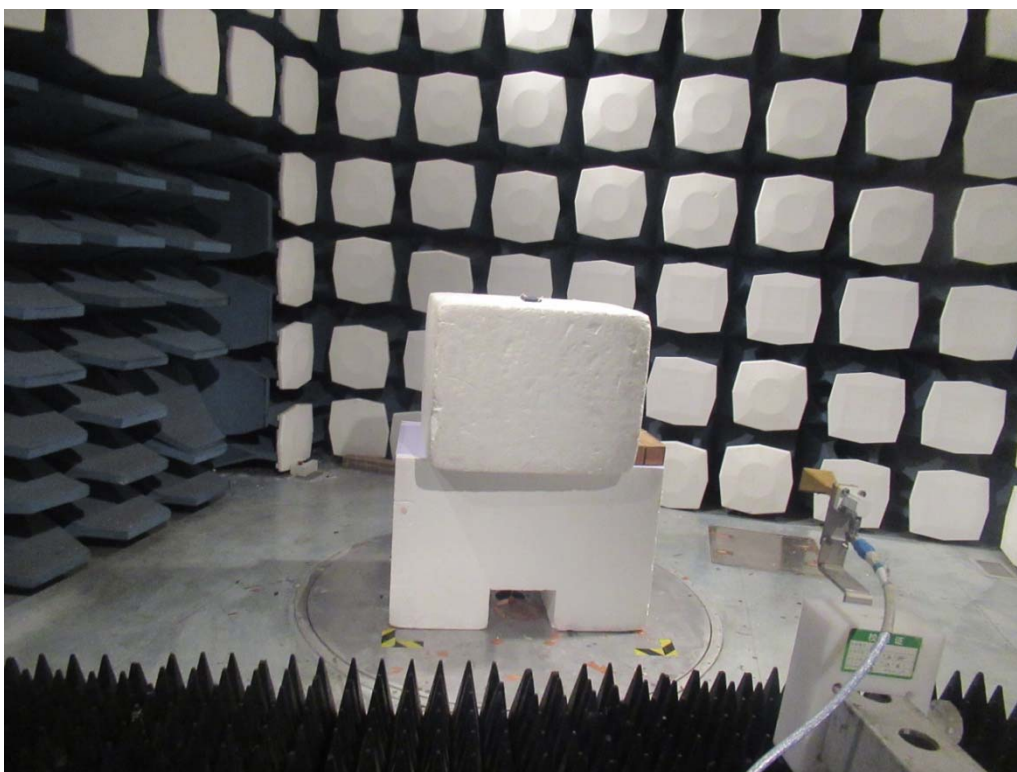
26.5GHz - 40GHz
