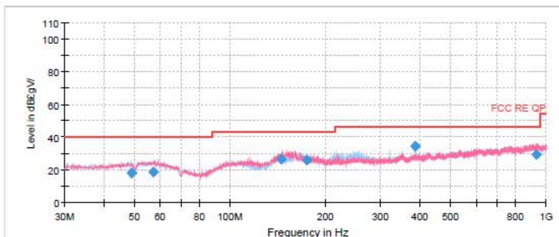
Radiated Emission from 30MHz to 1GHz
