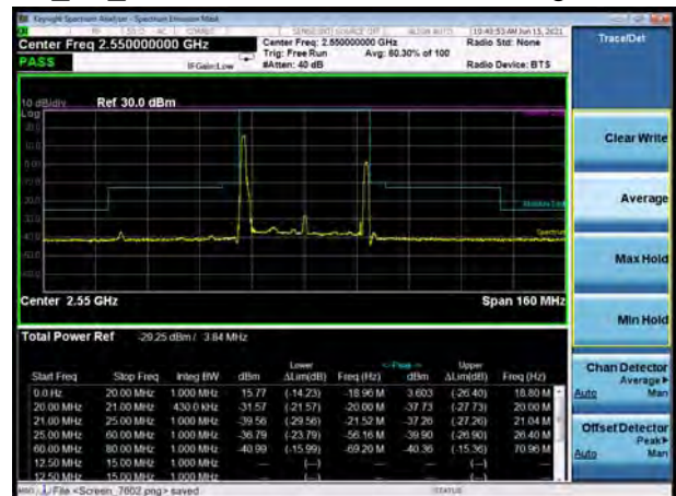
CA_7C_20MHz+20MHz 64QAM CH- High, RB 1
