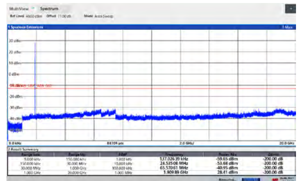
GPRS 1900 CH-High 9kHz ~ 20GHz
