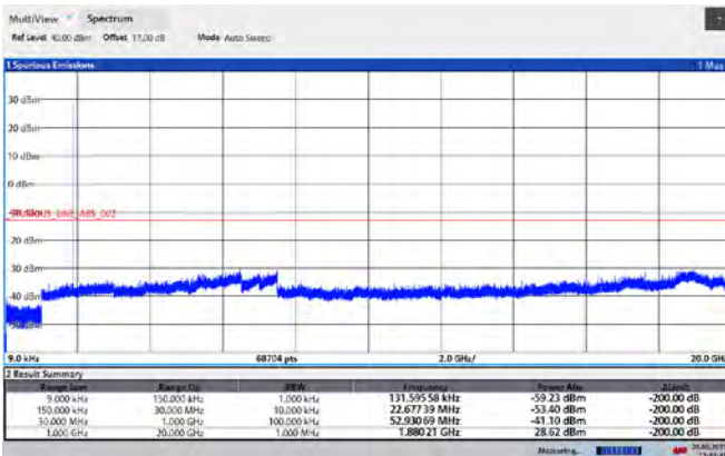
GSM 1900 CH- Middle 9kHz ~ 20GHz
