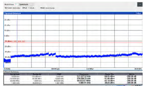
GPRS 1900 CH- Middle 9kHz ~ 20GHz
