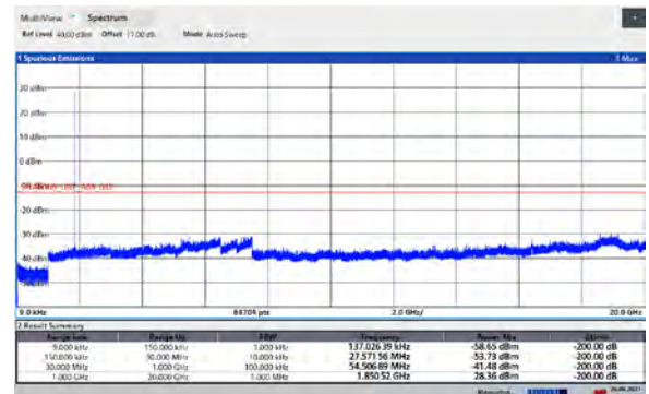
GSM 1900 CH-Low 9kHz ~ 20GHz
