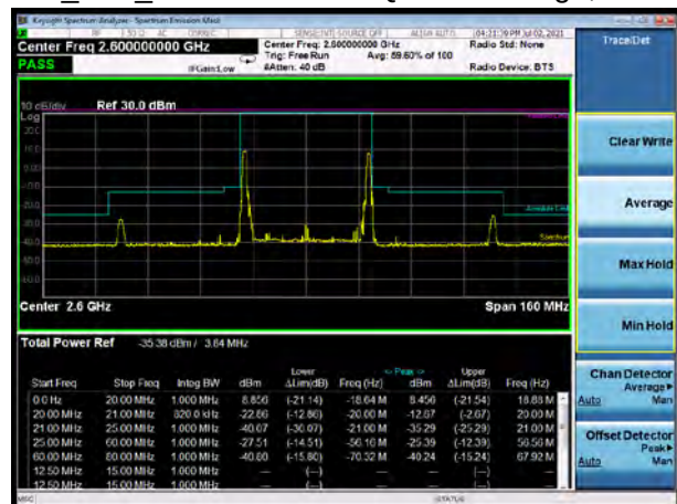
CA_38C_20MHz+20MHz 16QAM CH- High, RB 1
