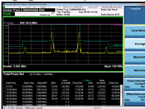
CA_38C_15MHz+15MHz QPSK CH-Low, RB 1
