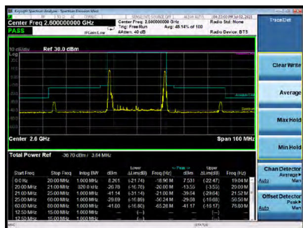
CA_38C_20MHz+20MHz 64QAM CH- High, RB 1
