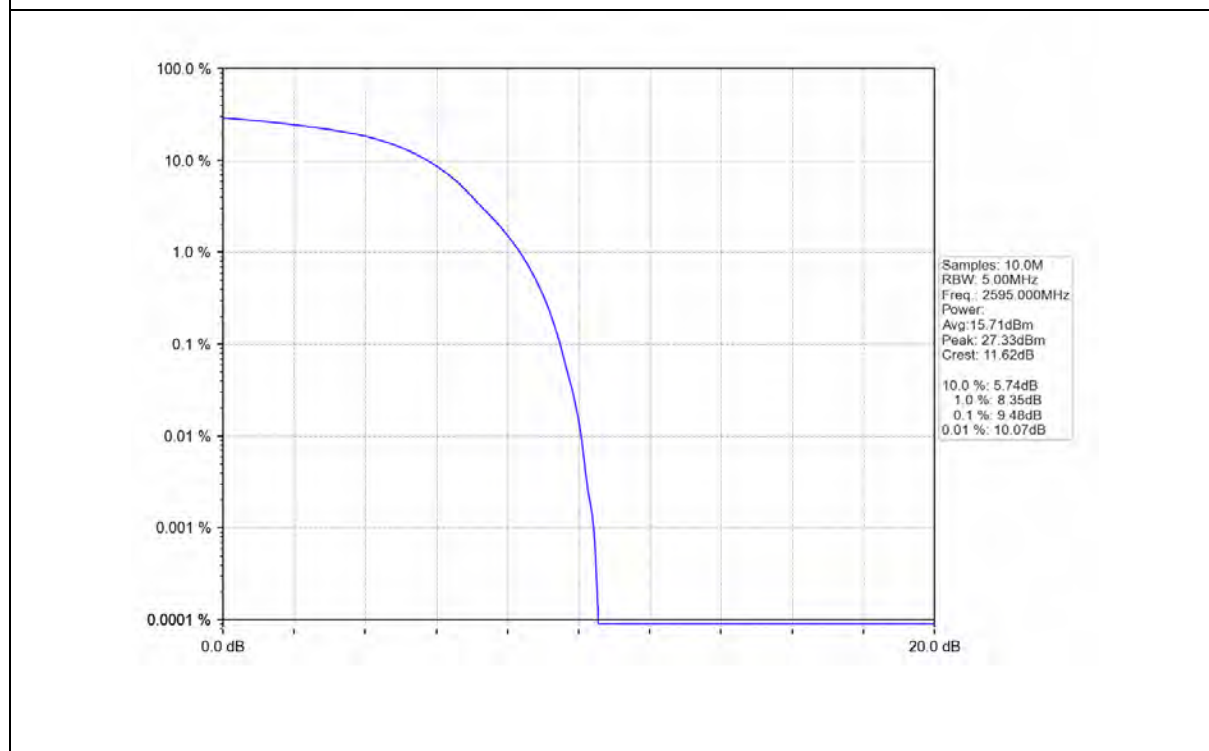
Band38_15MHz_QPSK_MCH_2595MHz_RB_75_0_NTNV
