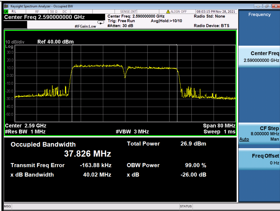
Band_38C_20MHz+20MHz_16QAM_MCH_NTNV
