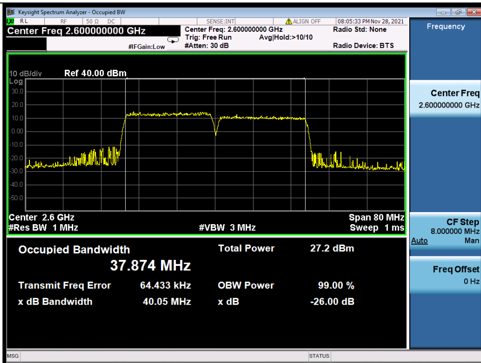
Band_38C_20MHz+20MHz_16QAM_LCH_NTNV
