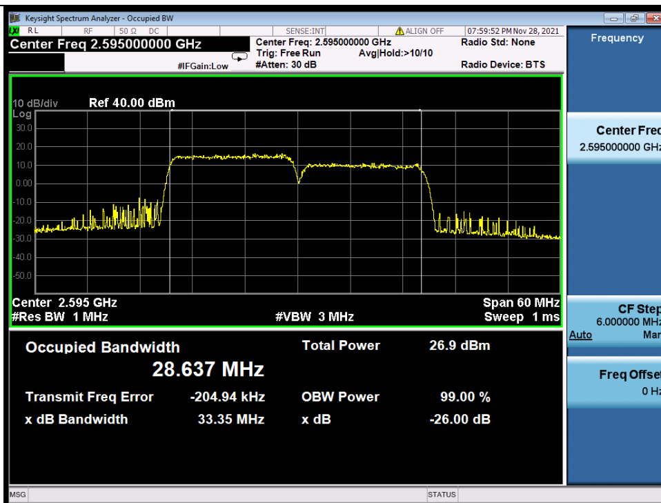
Band_38C_15MHz+15MHz_16QAM_HCH_NTNV
