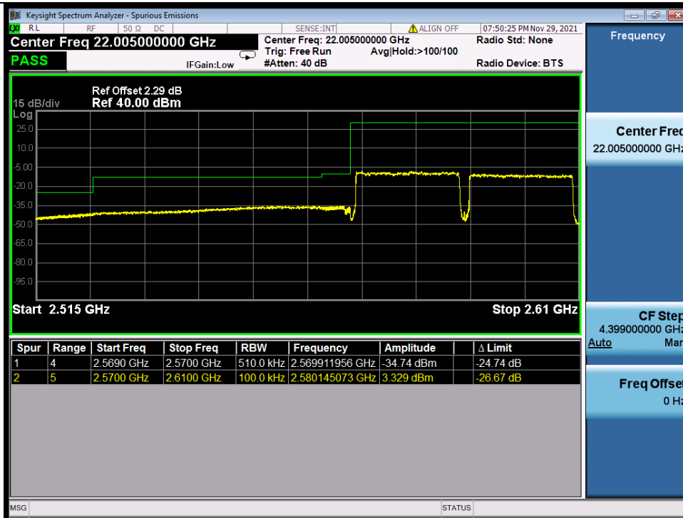
Band_38C_64QAM_HCH_20M+20M_RB_1_0/1_99_NTNV
