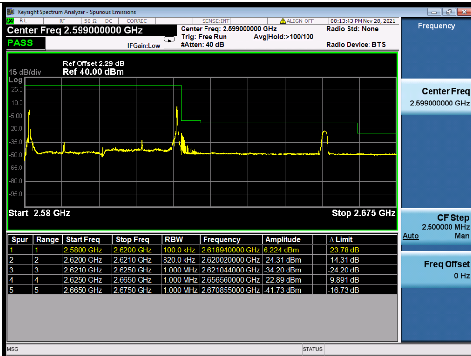
Band_38C_16QAM_HCH_20M+20M_RB_1_99/1_0_NTNV
