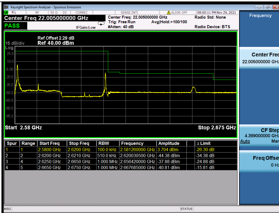
Band_38C_64QAM_HCH_20M+20M_RB_1_99/1_0_NTNV
