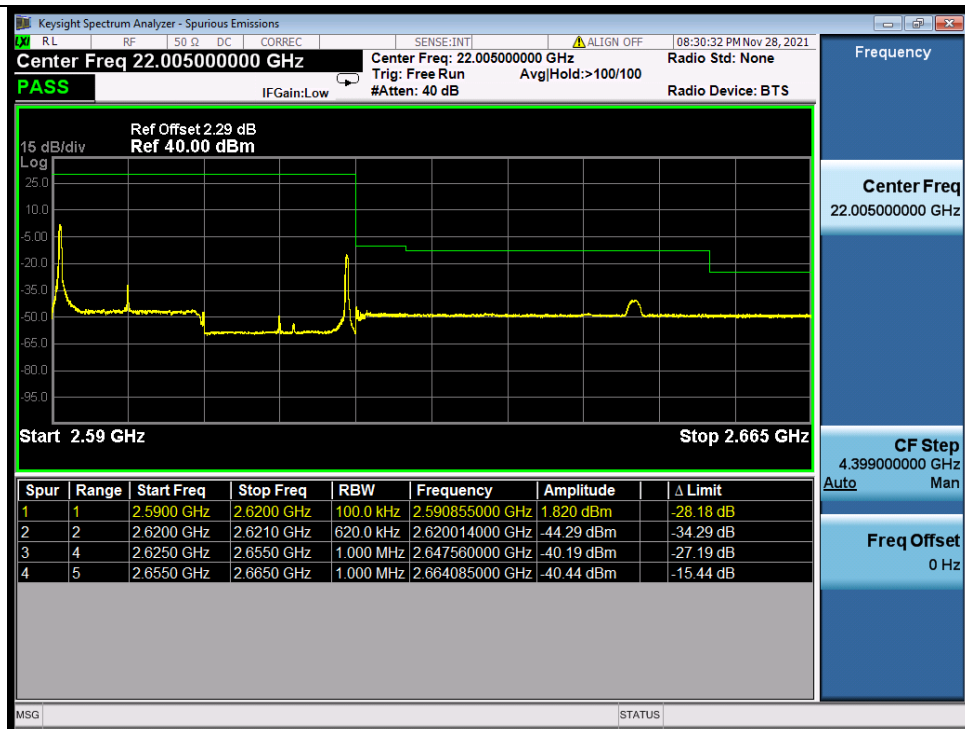
Band_38C_QPSK_HCH_15MHz+15MHz_RB_1_74/1_0_NTNV
