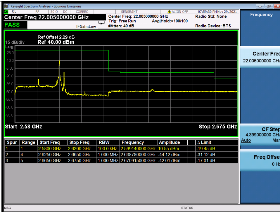
Band_38C_64QAM_HCH_20M+20M_RB_FULL_0_NTNV
