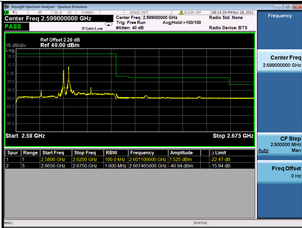
Band_38C_16QAM_HCH_20M+20M_RB_FULL_0_NTNV
