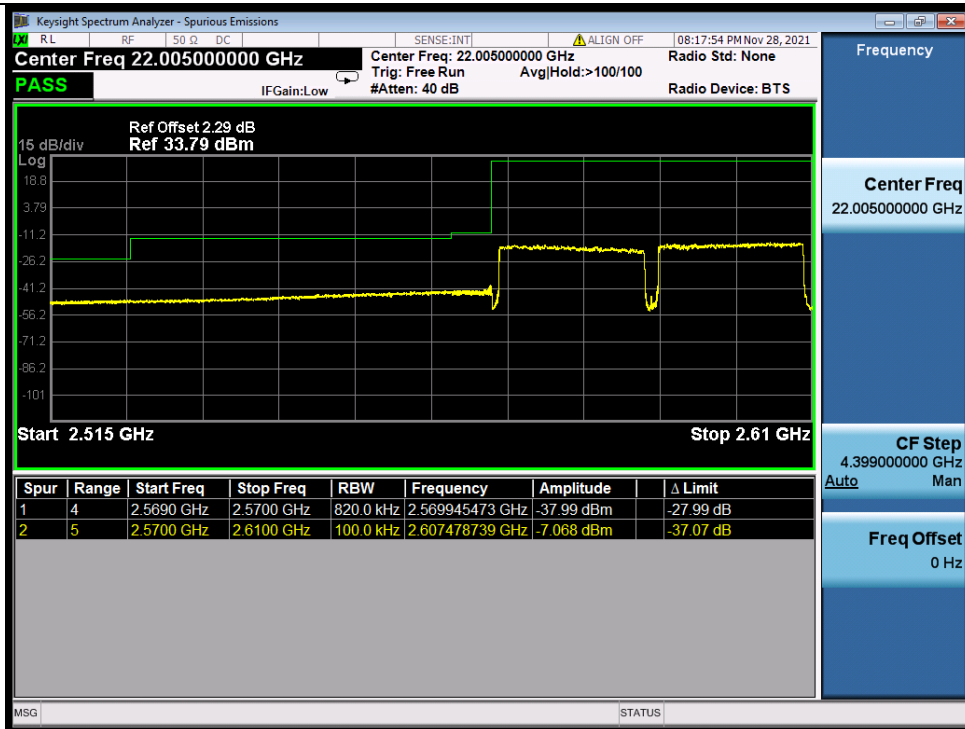
Band_38C_16QAM_HCH_20M+20M_RB_1_0/1_99_NTNV
