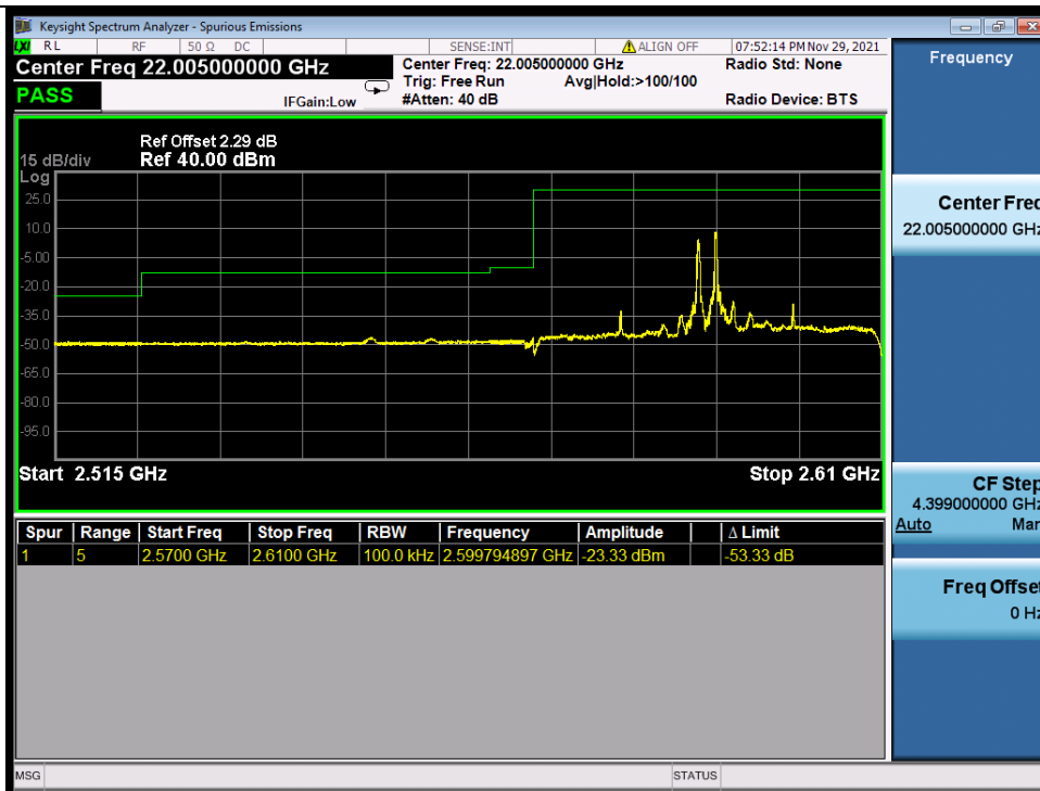
Band_38C_64QAM_LCH_20M+20M_RB_FULL_0_NTNV
