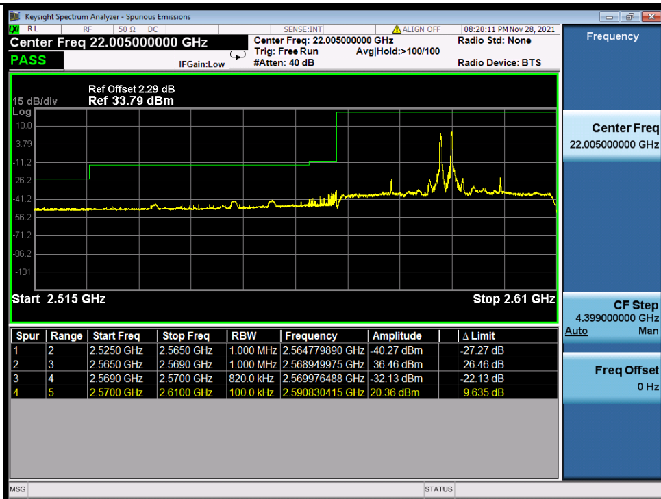
Band_38C_16QAM_LCH_20M+20M_RB_FULL_0_NTNV
