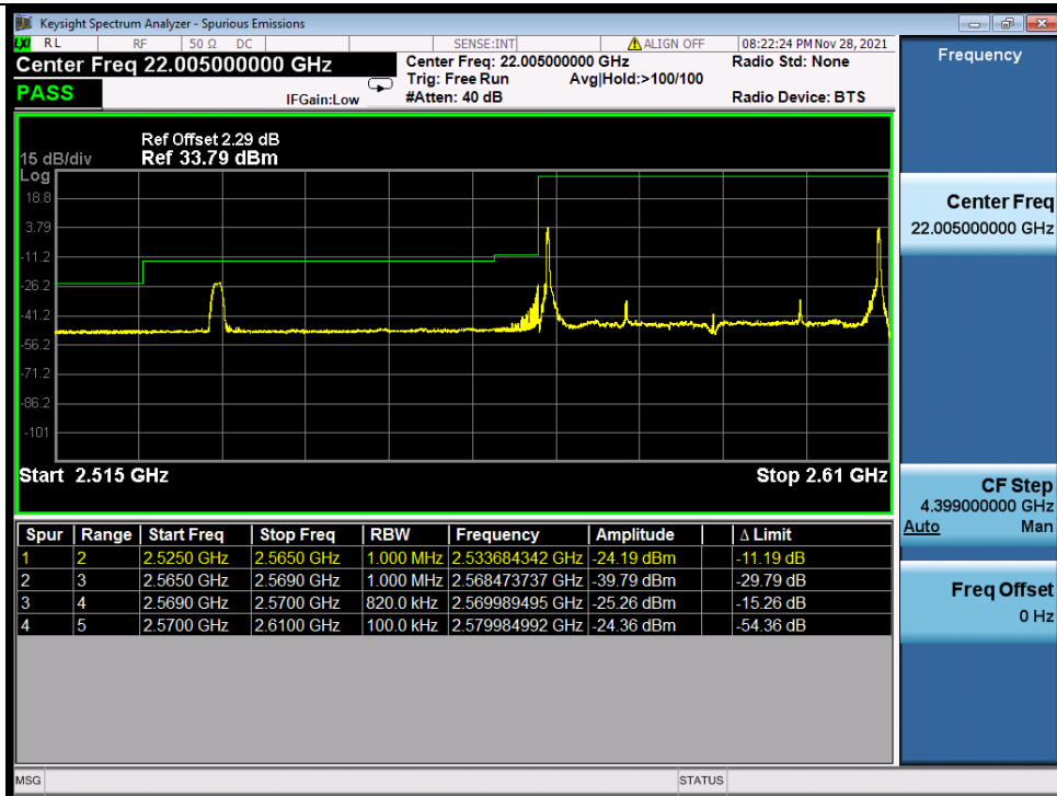
Band_38C_16QAM_LCH_20M+20M_RB_1_99/1_0_NTNV
