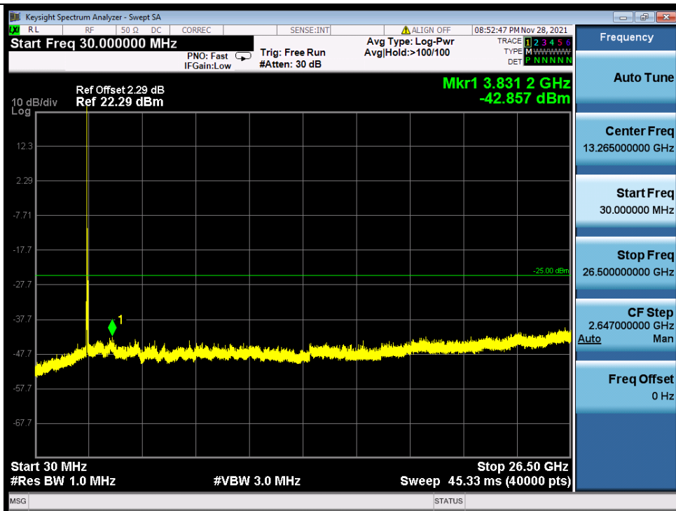
Band_38C_16QAM_LCH_20M+20M_RB_1_0/1_99_NTNV
