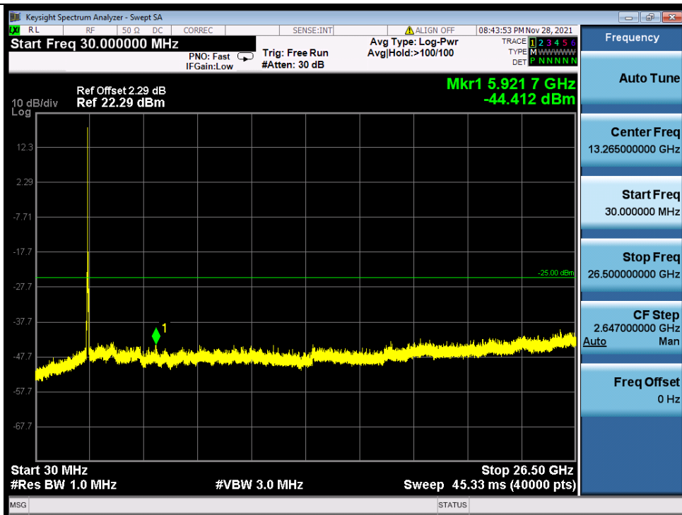
Band_38C_QPSK_HCH_15MHz+15MHz_RB_1_0/1_74_NTNV
