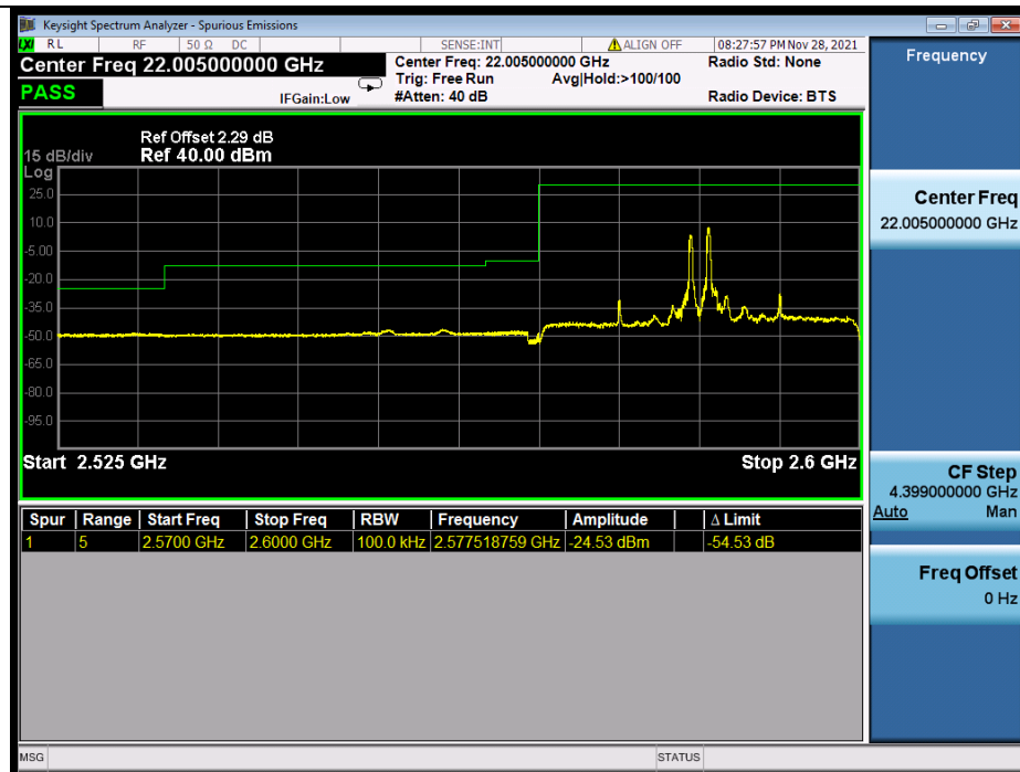
Band_38C_QPSK_LCH_15MHz+15MHz_RB_FULL_0_NTNV
