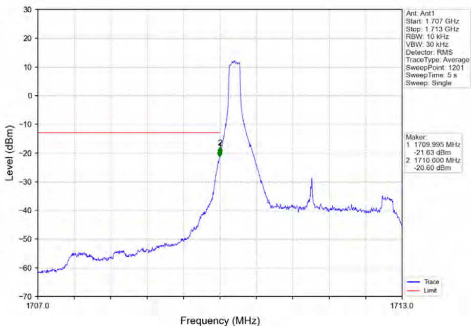
Band4_3MHz_QPSK_LCH_1711.5MHz_RB_1_0_NTNV
