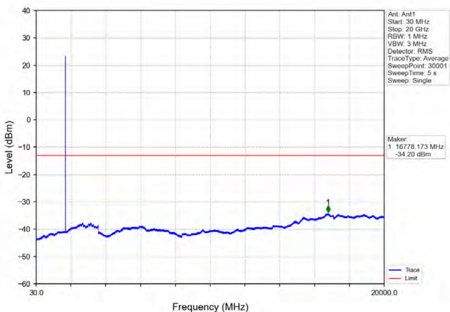
Band4_3MHz_QPSK_LCH_1711.5MHz_RB_1_0_NTNV
