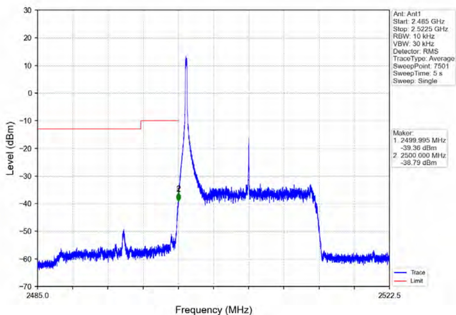
Band7_15MHz_QPSK_LCH_2507.5MHz_RB_1_0_NTNV
