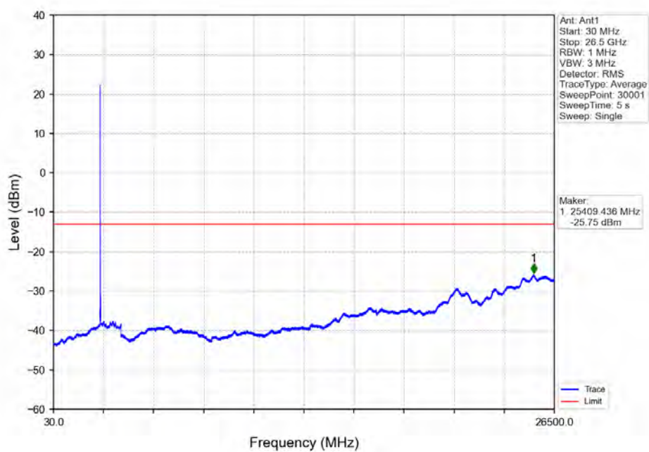
Band7_15MHz_QPSK_LCH_2507.5MHz_RB_1_0_NTNV
