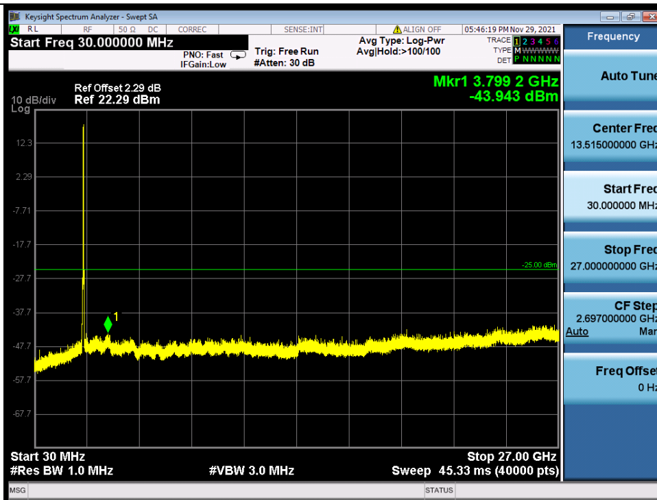
Band_7C_16QAM_LCH_15M+15M_RB_1_0/1_74_NTNV
