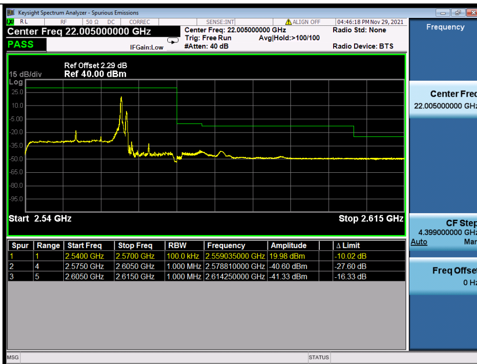
Band_7C_64QAM_HCH_20M+10M_RB_FULL_0_NTNV
