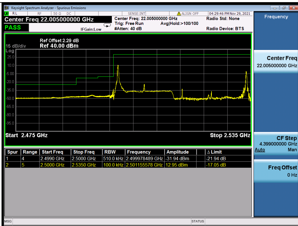
Band_7C_64QAM_LCH_15M+20M_RB_1_74/1_0_NTNV
