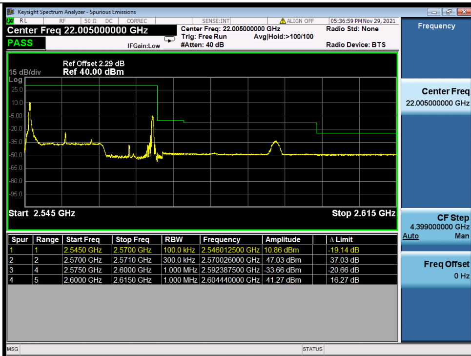
Band_7C_16QAM_HCH_15M+10M_RB_1_74/1_0_NTNV
