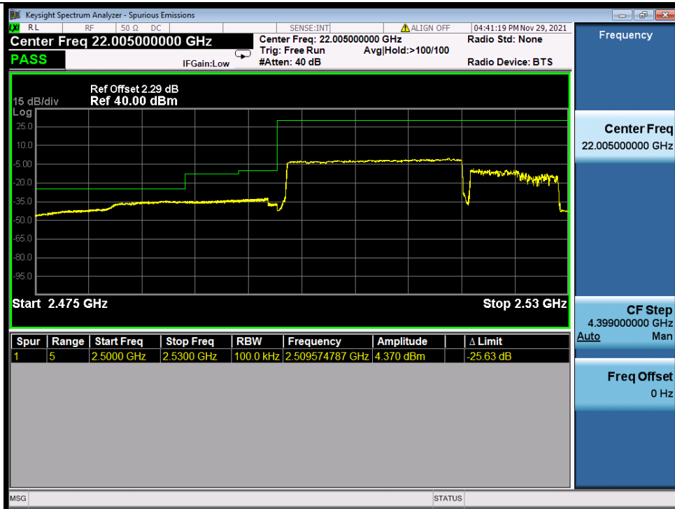
Band_7C_16QAM_LCH_20M+10M_RB_1_99/1_0_NTNV
