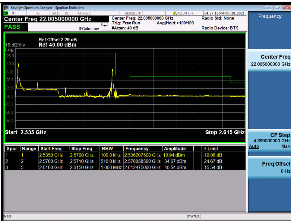
Band_7C_QPSK_HCH_15M+20M_RB_1_74/1_0_NTNV
