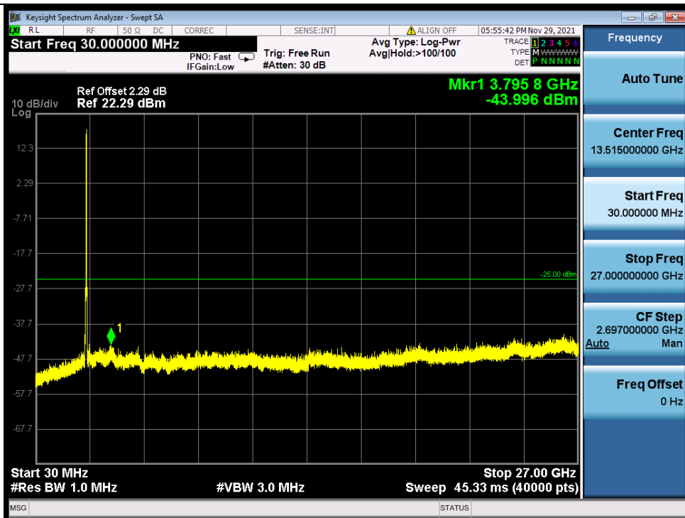
Band_7C_16QAM_LCH_20M+10M_RB_1_0/1_49_NTNV
