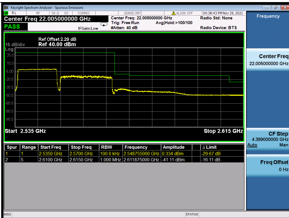
Band_7C_64QAM_LCH_15M+20M_RB_1_0/1_99_NTNV
