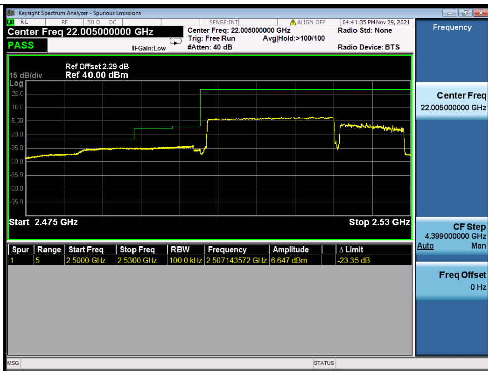
Band_7C_64QAM_HCH_20M+10M_RB_1_0/1_49_NTNV
