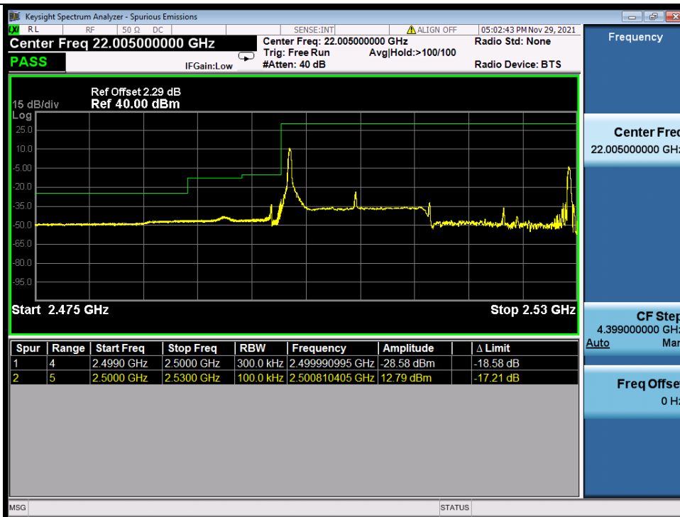
Band_7C_16QAM_LCH_15M+15M_RB_1_74/1_0_NTNV
