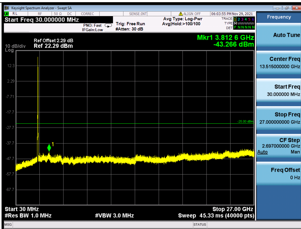
Band_7C_QPSK_HCH_15M+20M_RB_1_0/1_99_NTNV
