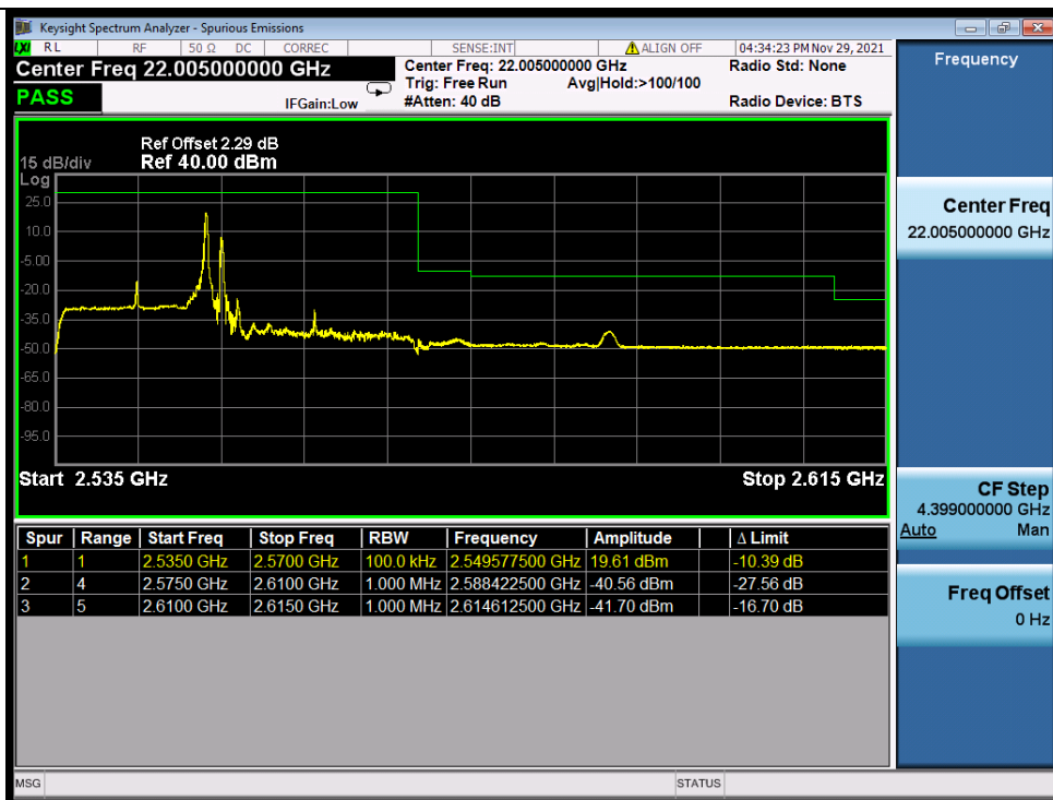
Band_7C_64QAM_HCH_15M+20M_RB_FULL_0_NTNV
