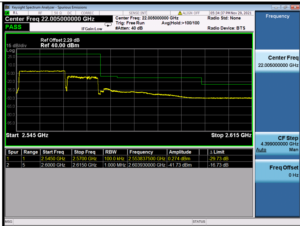
Band_7C_QPSK_HCH_15M+10M_NTNV
