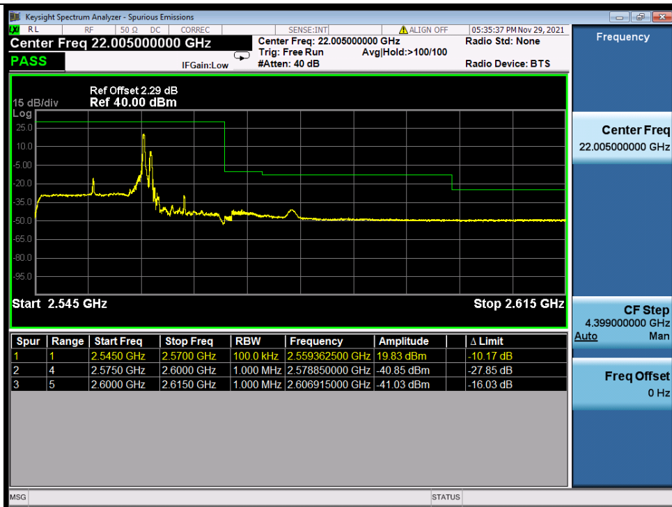
Band_7C_QPSK_HCH_15M+10M_RB_FULL_0_NTNV
