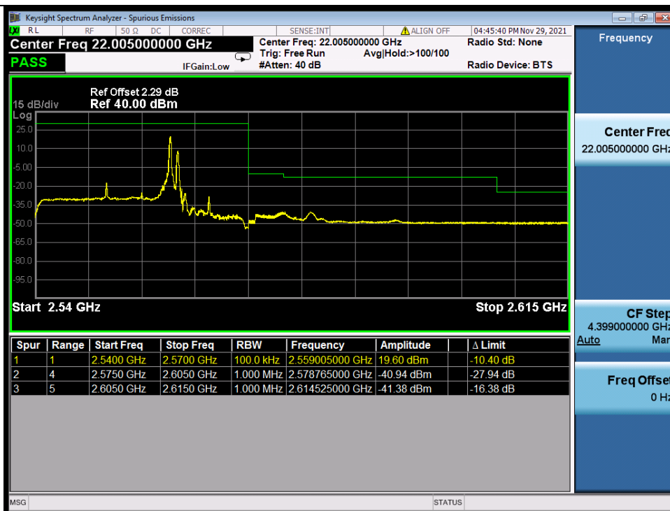
Band_7C_QPSK_HCH_20M+10M_RB_FULL_0_NTNV
