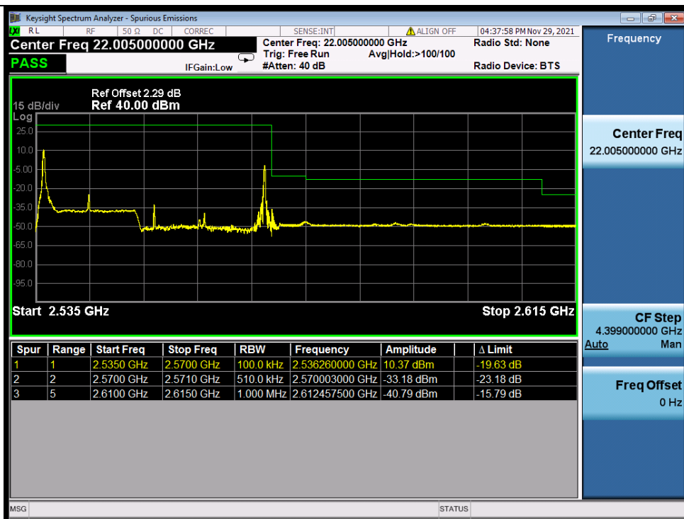
Band_7C_64QAM_HCH_15M+20M_RB_1_74/1_0_NTNV
