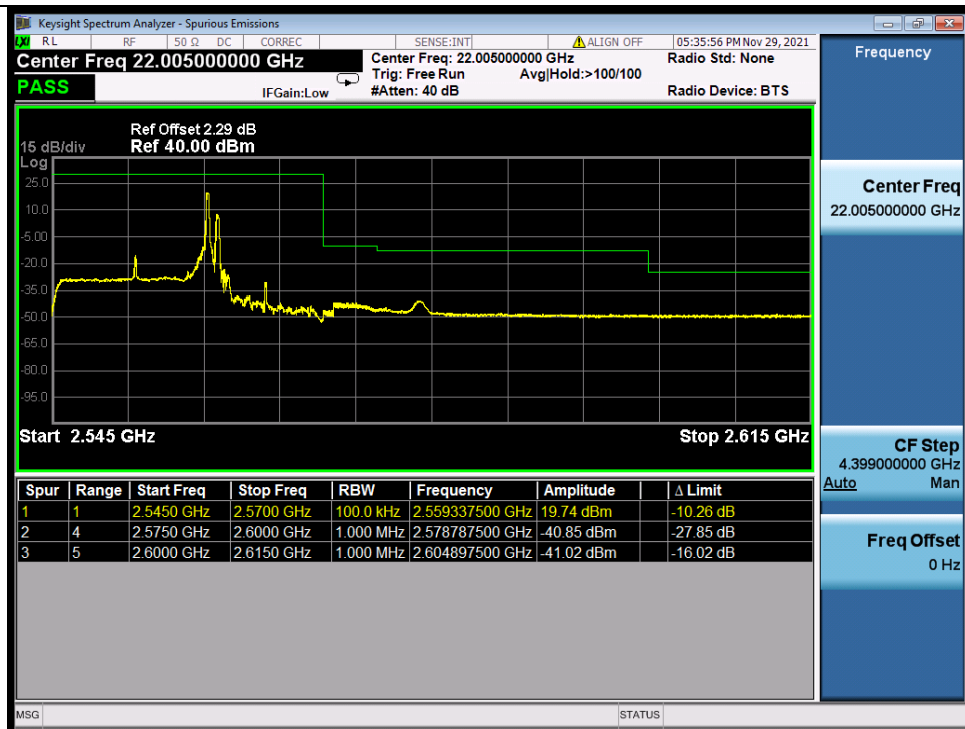
Band_7C_16QAM_HCH_15M+10M_RB_FULL_0_NTNV
