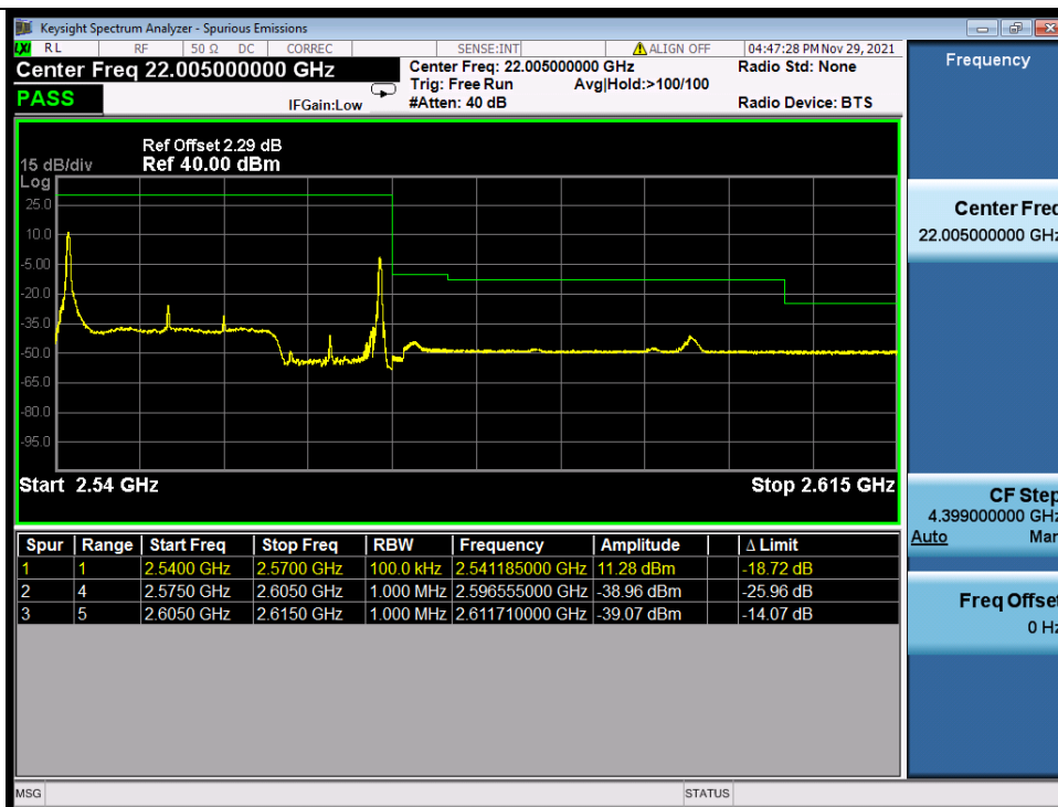
Band_7C_64QAM_HCH_20M+10M_RB_1_99/1_0_NTNV
