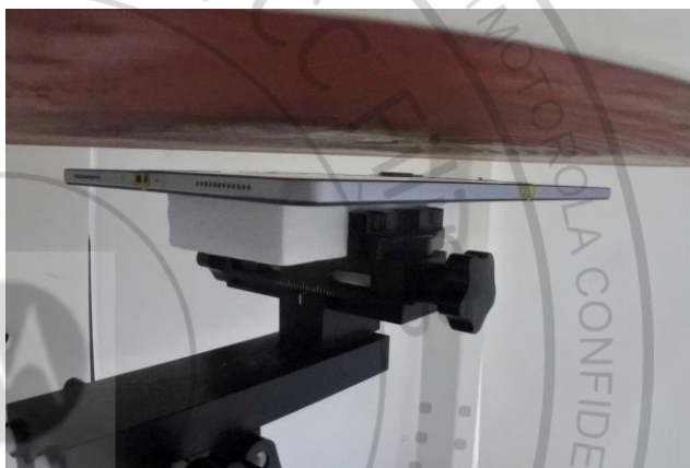
Bottom Face, Test Separation 10 mm (Sensor off)
