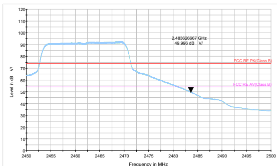
802.11g-Channel 11 Average
