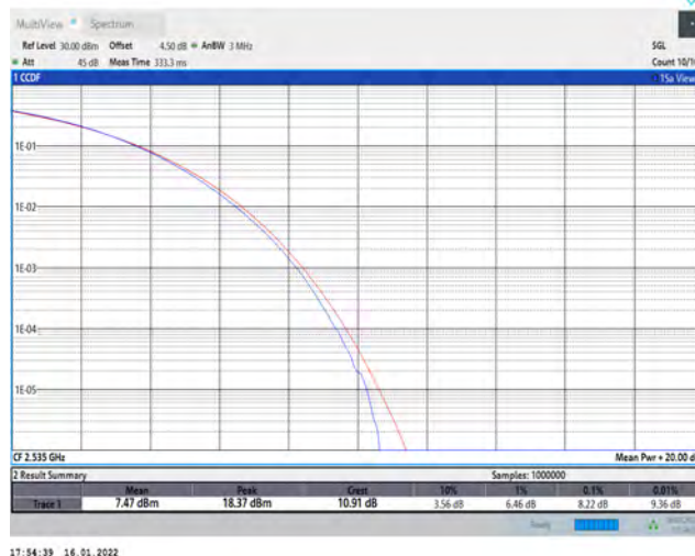
CA_7C-20MHz-20MHz-QPSK-QPSK-21001-21199-100RB#0-100RB#0
